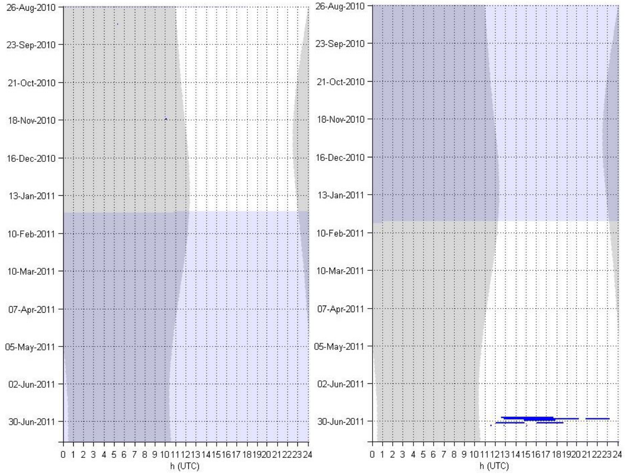
Explosions – Occurrence in hourly bins at sites A (left panel) and B (right panel).
