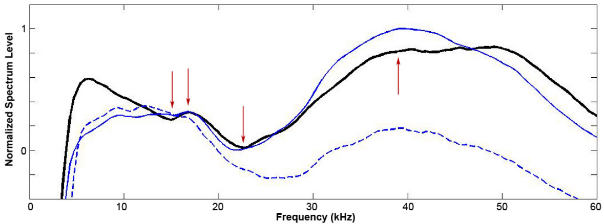
Figure 29. Mean Spectra of CT32. Example (black line), template (blue line), and noise floor (dotted line). Arrows are spectral peaks or troughs.
