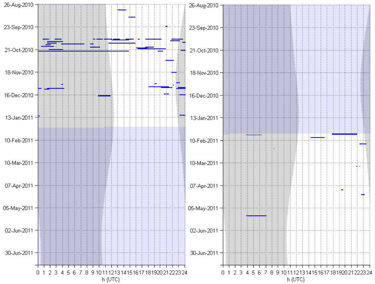
Mid-frequency active sonar – Occurrence in hourly bins at sites A (left panel) and B (right panel).
