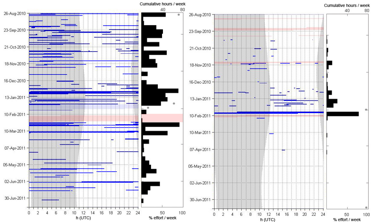
Figure 46. CT26 echolocation clicks in one-minute bins (blue) and weekly (black) at site A (left) and site B (right) between August 2010 and July 2011. Red shading indicates data gaps. Gray shading is nighttime.
