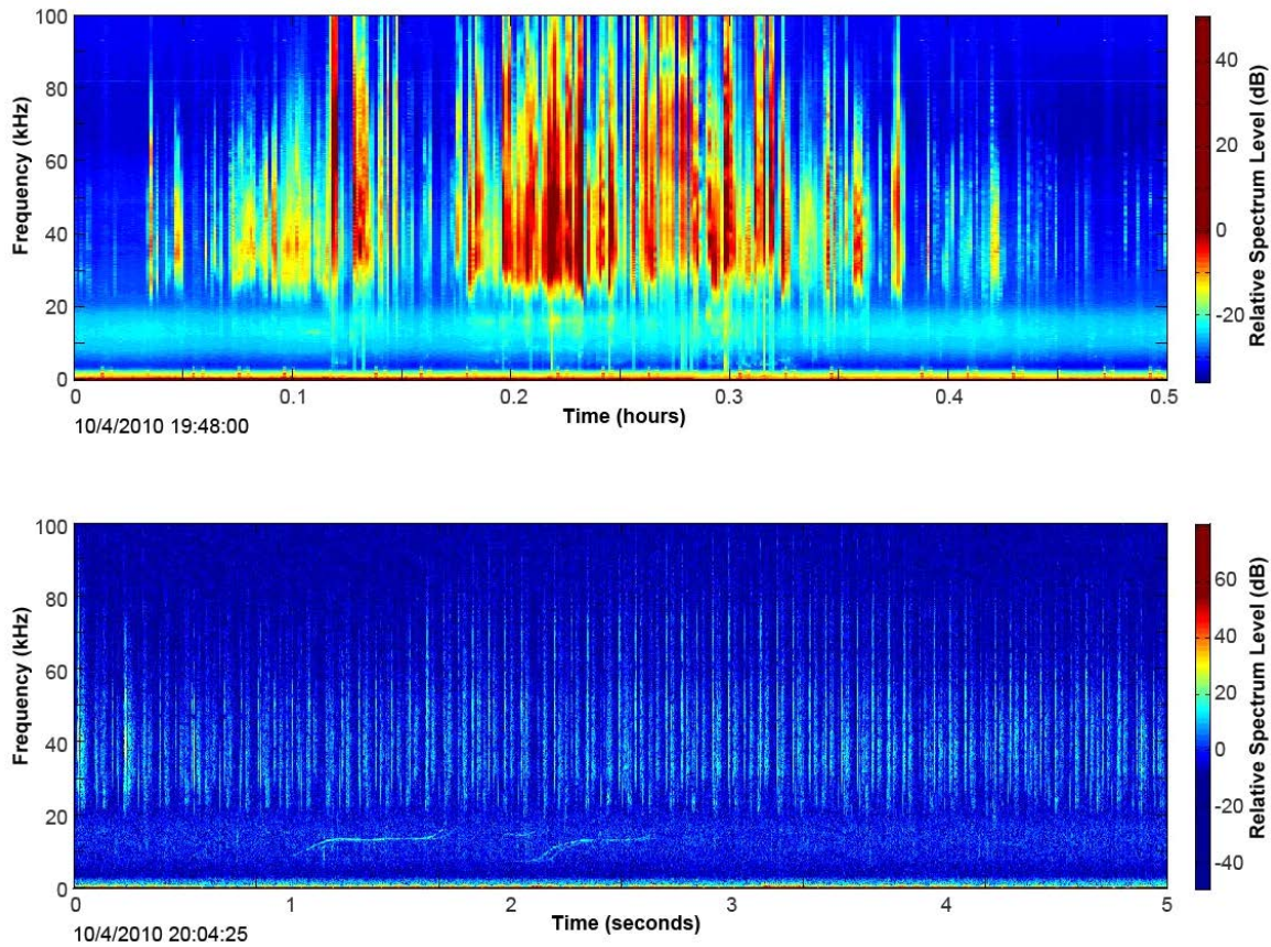
Figure 26. CT30 in the LTSA (above) and spectrogram (below).
