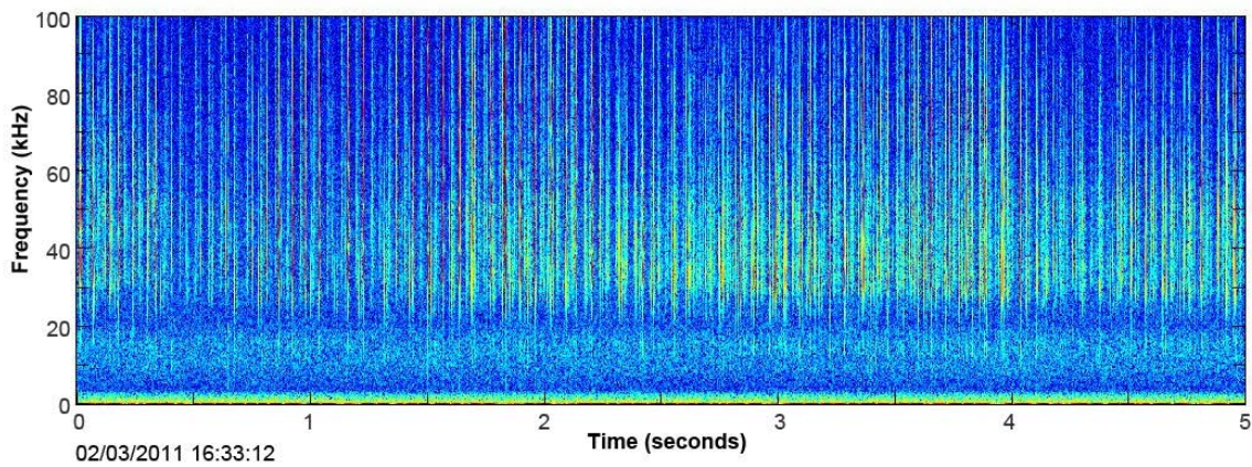
Figure 20. CT25 in the LTSA (above) and spectrogram (below).
