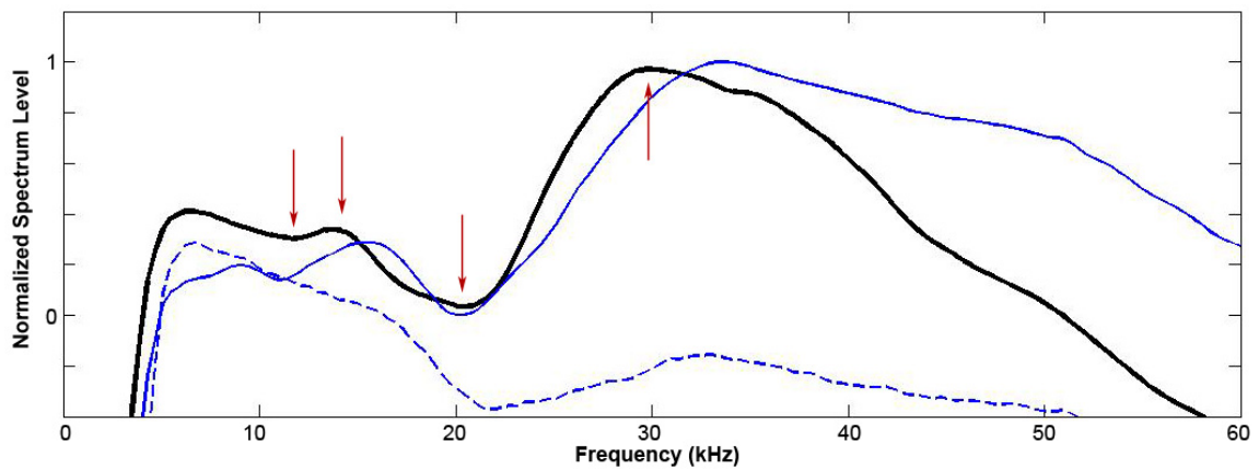
Figure 21. Mean Spectra of clicks for CT25. Example encounter (black line), template for CT (blue line; from G of Mex and/or North Carolina), noise floor (dotted line). Arrows are spectral peaks or troughs.
