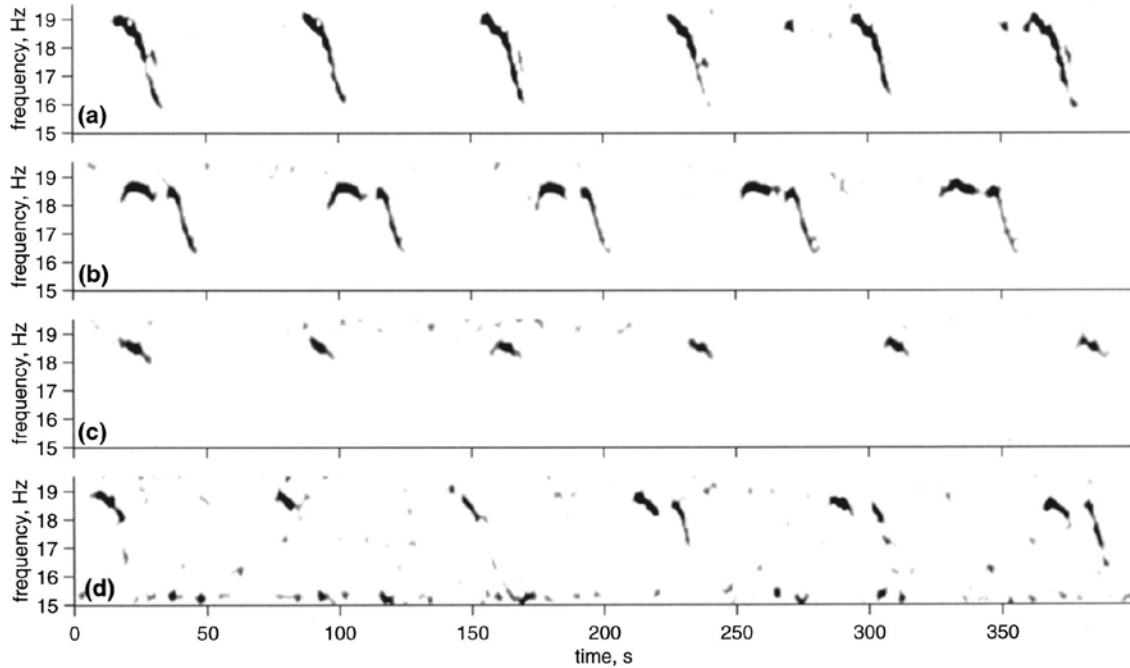
Figure 2. Blue whale A and B calls from Mellinger and Clark (2003).
