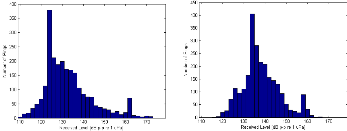
Figure 52. Distribution of MFA sonar pings by received level at site A (left) and site B (right) in 2 dB bins. Peak number of pings is 124 dB pp re 1 \mu Pa for site A and 134 dB pp re 1 \mu Pa for site B. Minimum level is 110 dB pp re 1 \mu Pa and is related to the detection threshold. Maximum level is 173dB pp re 1 \mu Pa for site A and 166 dB pp re 1 \mu Pa for site B, set by the clipping level of the HARP.
