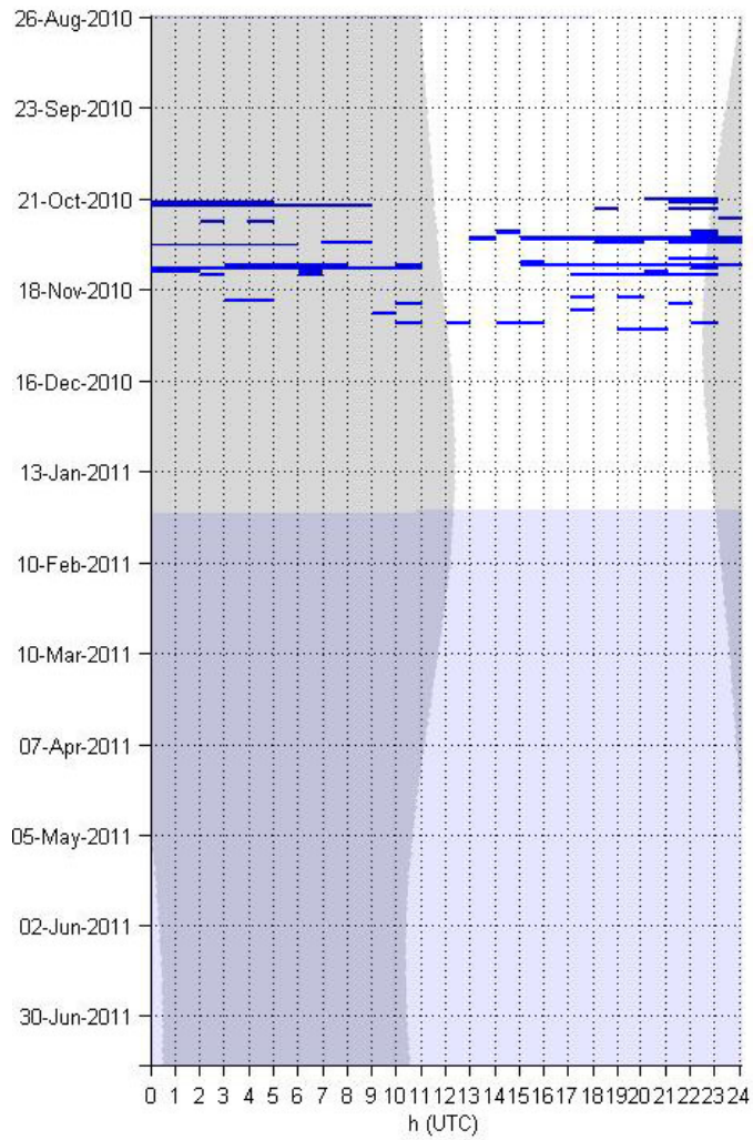
Unknown whale – 5-pulse calls in hourly bins at site A. No calls were detected at site B.
