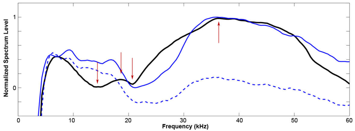
Figure 23. Mean Spectra of clicks for CT26. Example (black line), template (blue line), and noise floor (dotted line). Arrows are spectral peaks or troughs.
