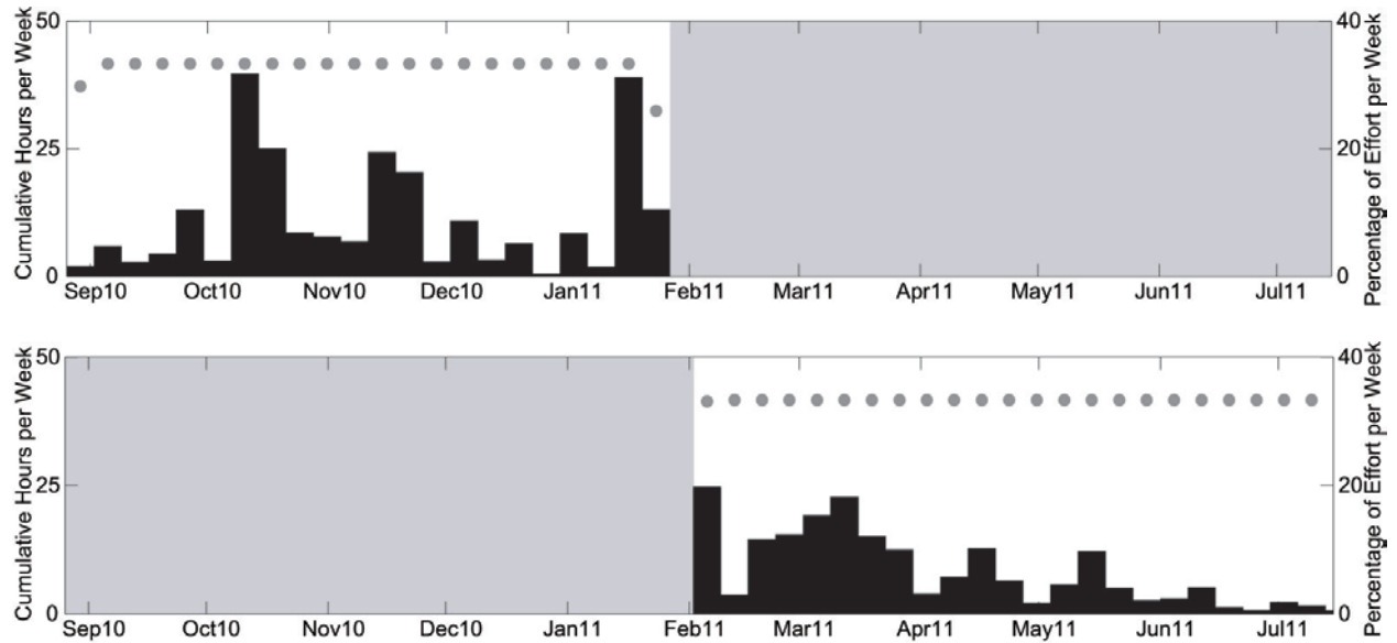
Figure 50. Broadband ship noise weekly hours at site A (top) and B (bottom) between August 2010 and July 2011. Effort markings are as described in Figure 35.
