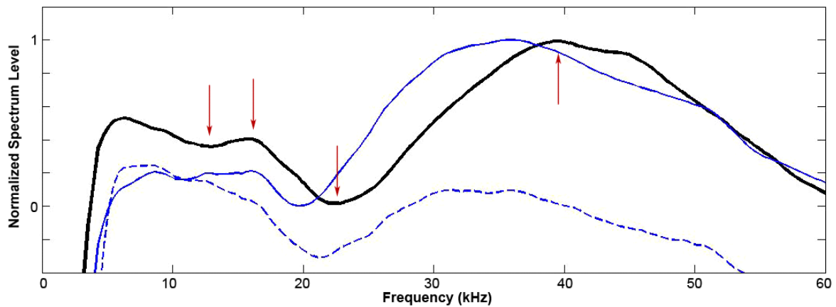
Figure 27. Mean Spectra of CT30. Example (black line), template (blue line), and noise floor (dotted line). Arrows are spectral peaks or troughs.
