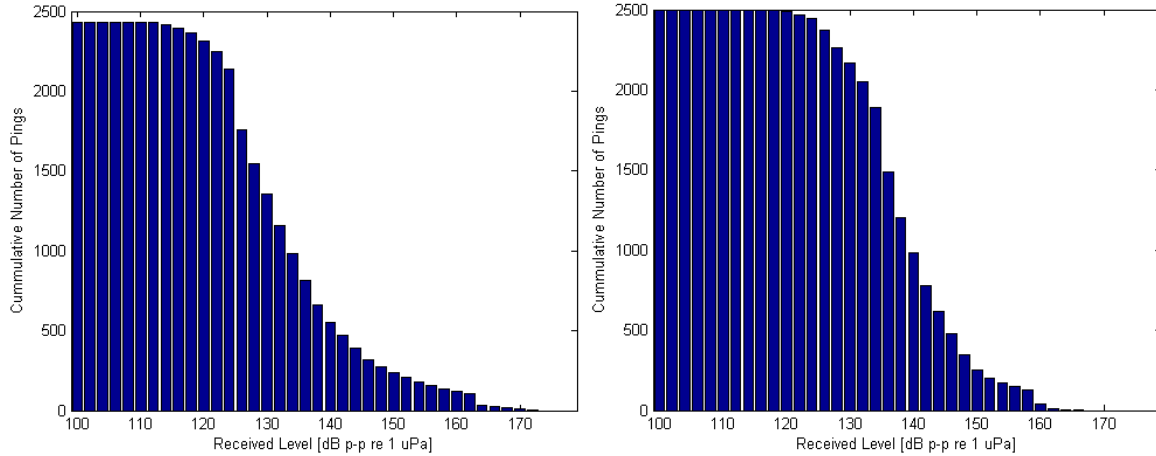
Figure 53. Cumulative distribution for the number of MFA sonar pings detected at a given received level or higher, at site A (left) and site B (right) in 2 dB bins.
