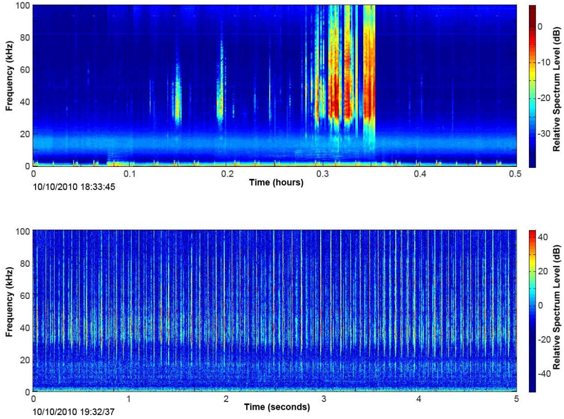
Figure 22. CT26 in the LTSA (above) and spectrogram (below).
