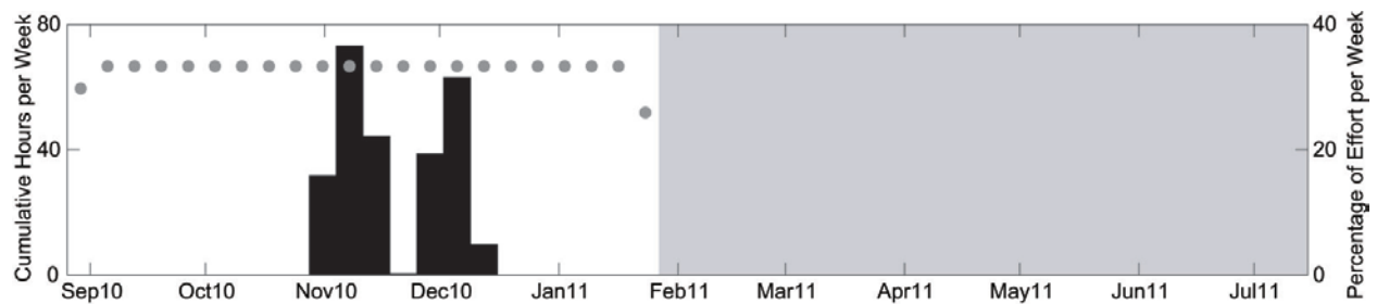
Figure 56. Weekly hours with 130-Hz tone detections at site A. Effort markings are as described in Figure 37.
