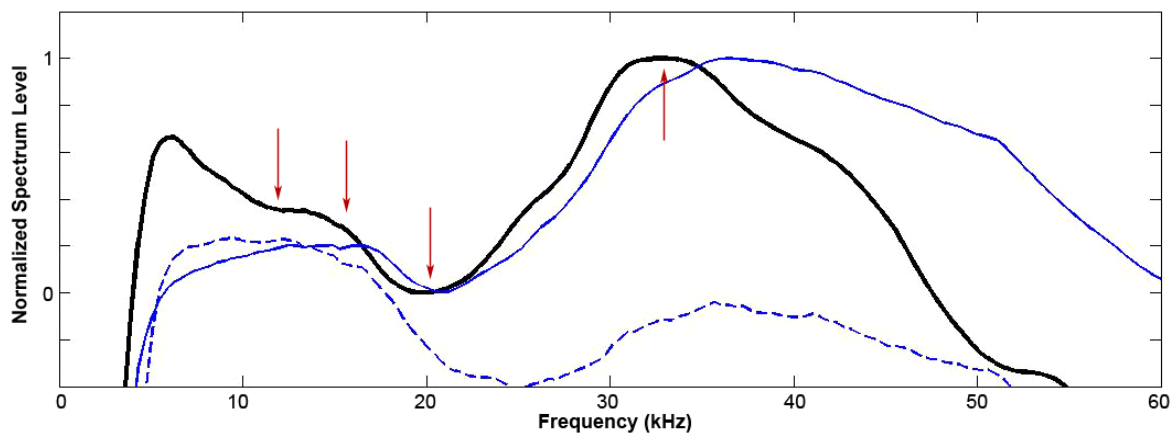
Figure 25. Mean spectra of CT27. Example (black line), template (blue line), and noise floor (dotted line). Arrows are spectral peaks or troughs.
