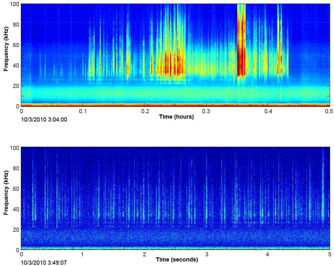
Figure 17. Risso's dolphin click bout in LTSA (above) and spectrogram (below). A distinctive banding pattern is seen in the LTSA.
