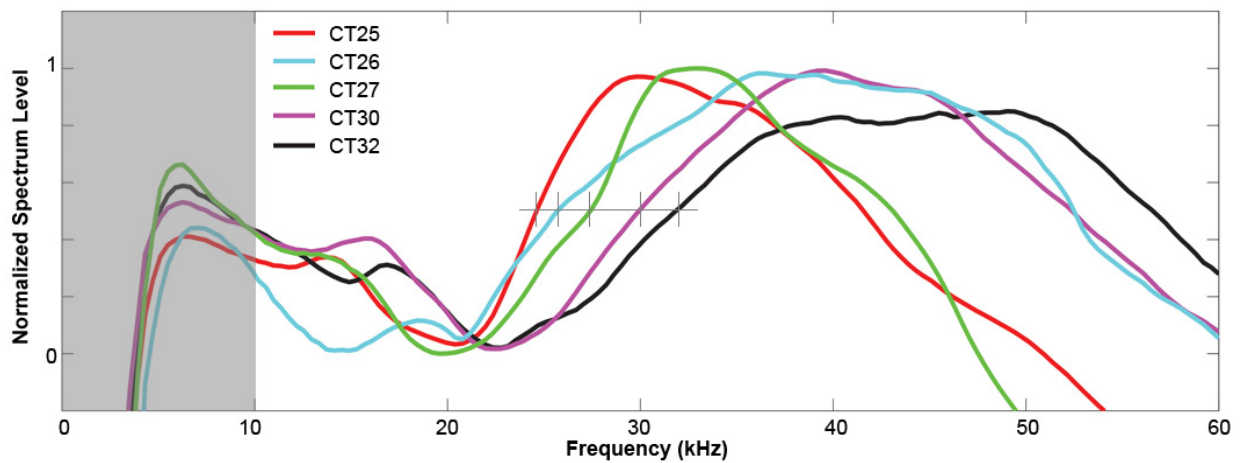
Figure 19. Echolocation click types (CT) that occurred in JAX recordings repeatedly. Numerical values (e.g. CT25 = 25 kHz) refers to low end of 50% energy bandwidth.
