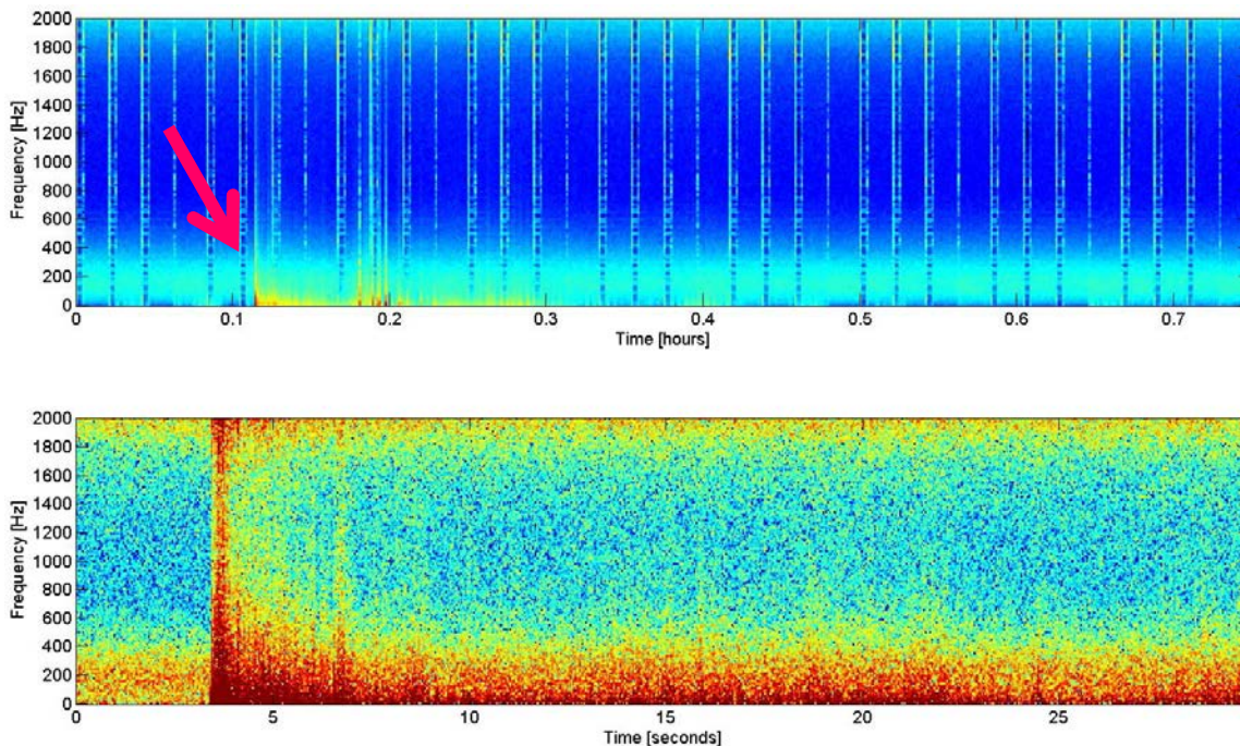
Figure 35. Five explosions are seen in the LTSA (arrow above) and one is expanded in the spectrogram (below). Site A on April 8, 2011.
