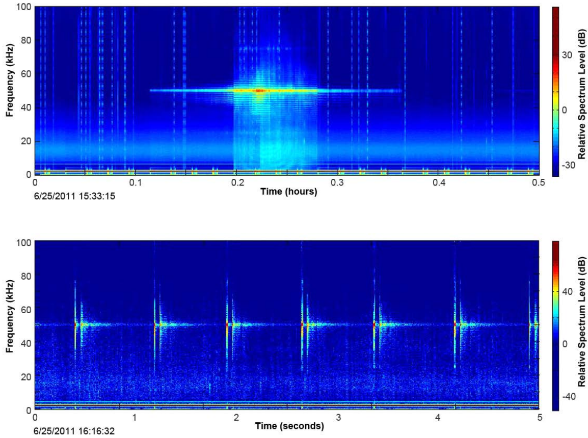
Figure 34. Echosounder in the LTSA (above) and spectrogram (below).
