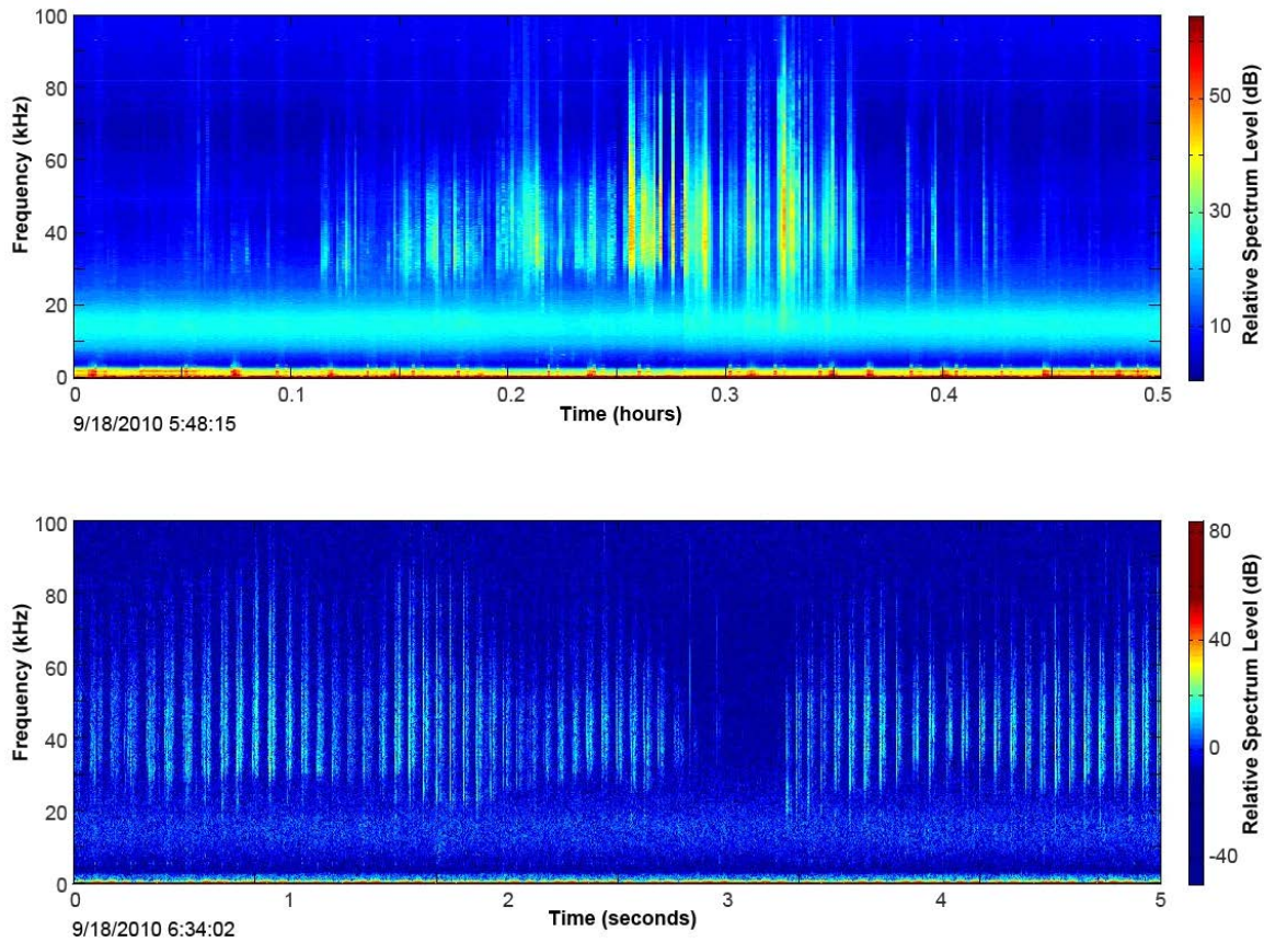
Figure 24. CT27 in the LTSA (above) and spectrogram (below).
