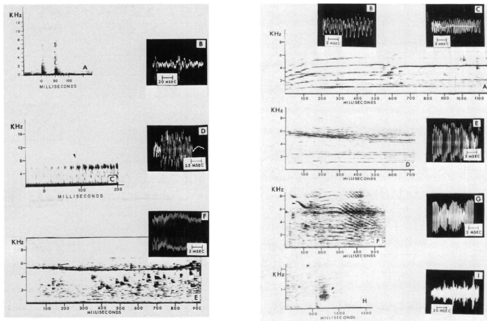
Figure 15. Killer whale vocalizations from Steiner et al. (1979).
