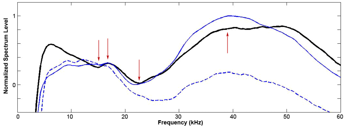
Figure 31. Mean Spectra of CT32. Example (black line), template (blue line), and noise floor (dotted line). Arrows are spectral peaks or troughs.
