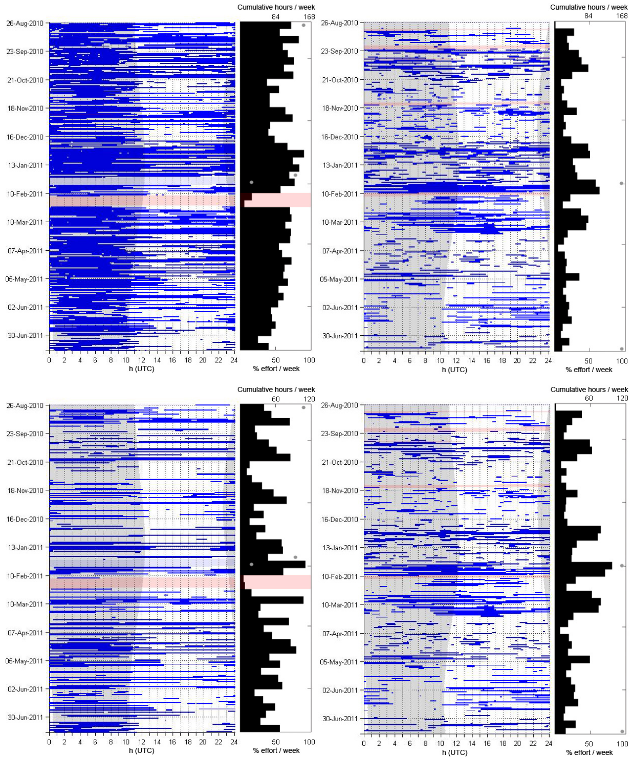
Figure 43. Odontocete echolocation clicks in one-minute bins (blue) and weekly presence (black) at site A (left) and site B (right) between August 2010 and July 2011. Top: all echolocation clicks of all species, Bottom: UO after all others were extracted. Red shading indicates data gaps. Gray shading is nighttime.
