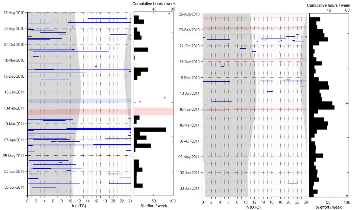
Figure 48. CT30 echolocation clicks in one-minute bins and weekly presence at site A (left) and site B (right) between August 2010 and July 2011. Red shading indicates data gaps. Gray shading is nighttime.
