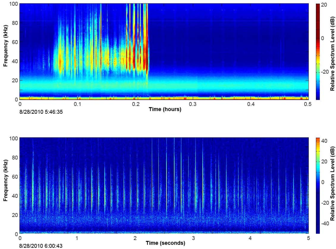
Figure 28. CT32 in the LTS A (above) and spectrogram (below).
