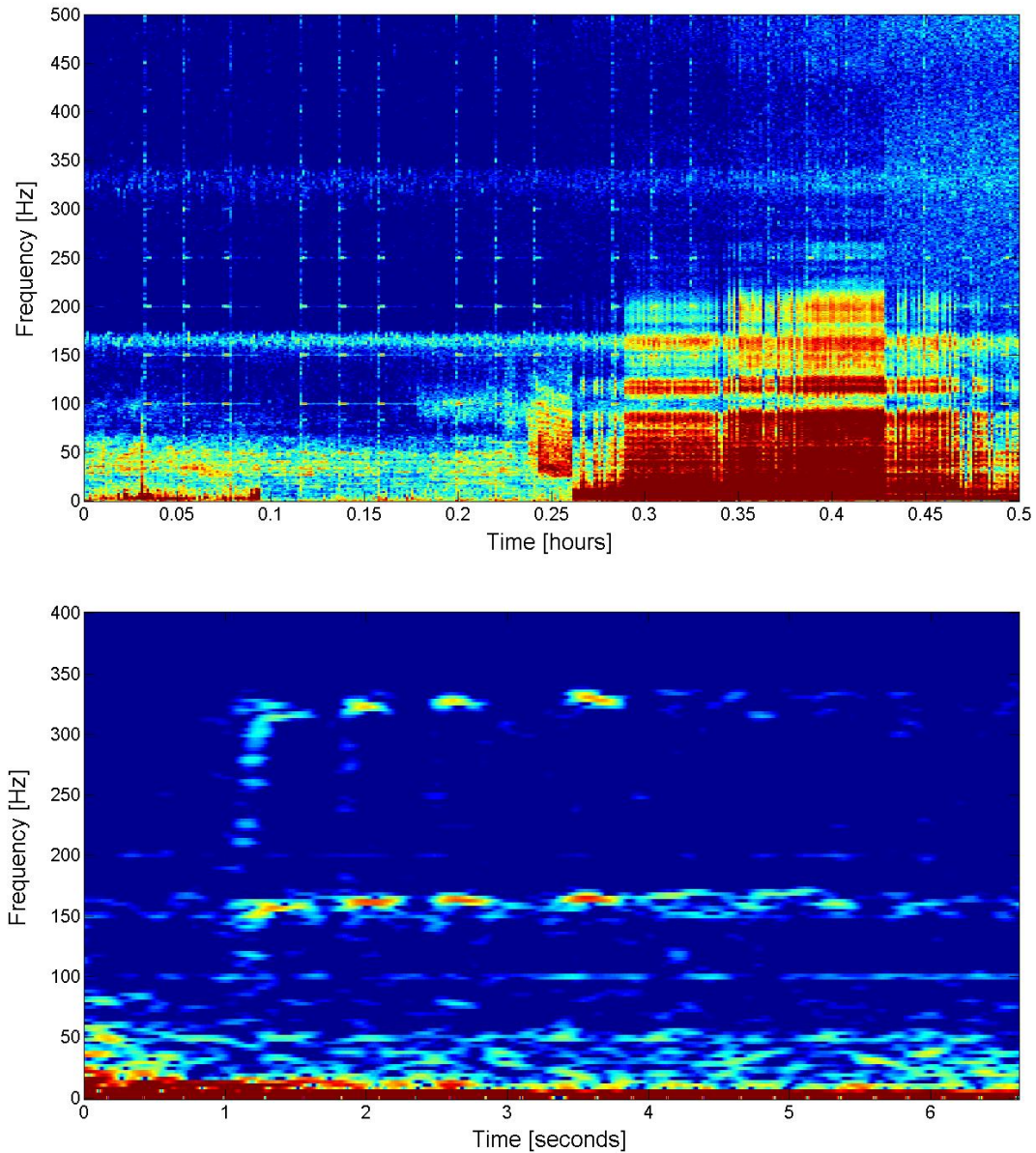
Figure 12. LTSA (top) of a band of 5 pulse calls and a spectrogram (bottom) of a single 5 pulse call (750-point FFT, 98% overlap) recorded on 26 August 2010 at site A.
