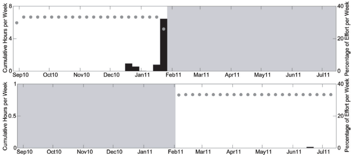
Figure 39. Weekly occurrence of minke speed-up/slow-down whale pulse trains at 150 Hz at site A (top) and site B (bottom). Effort as described in Figure 37
