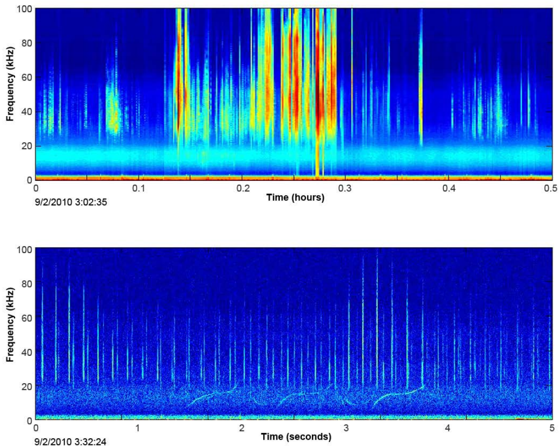
Figure 16. LTSA (top) and spectrogram (bottom) of odontocete echolocation clicks and whistles.
