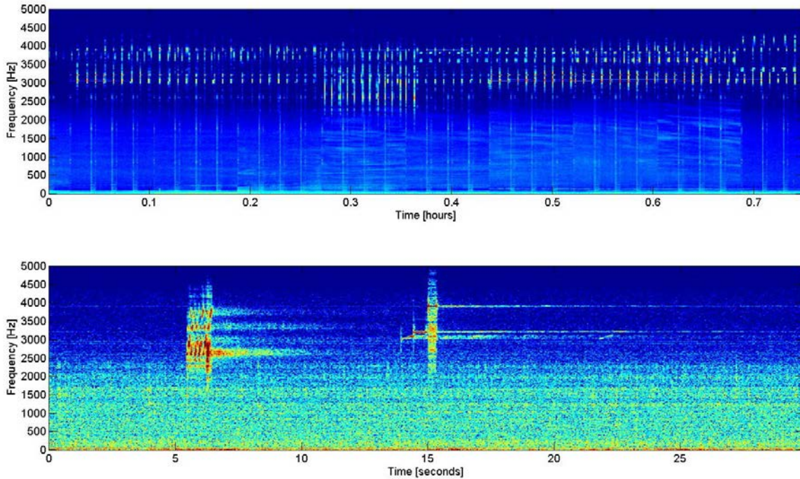
Figure 33. Mid-frequency active (MFA) sonar event. (Top) Long-Term Spectral Average of 45 minutes of data. (Bottom) Spectrogram of with multiple sonar pings.
