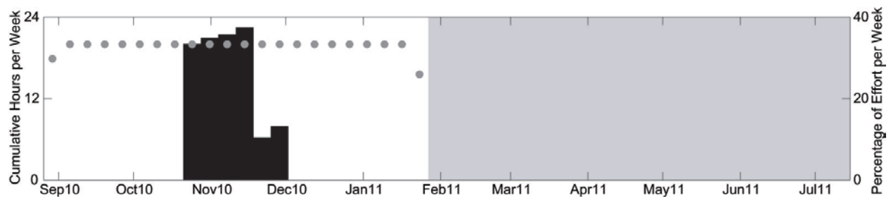
Figure 41. Weekly occurrence of 5-pulse calls at site A. Effort as described in Figure 37
