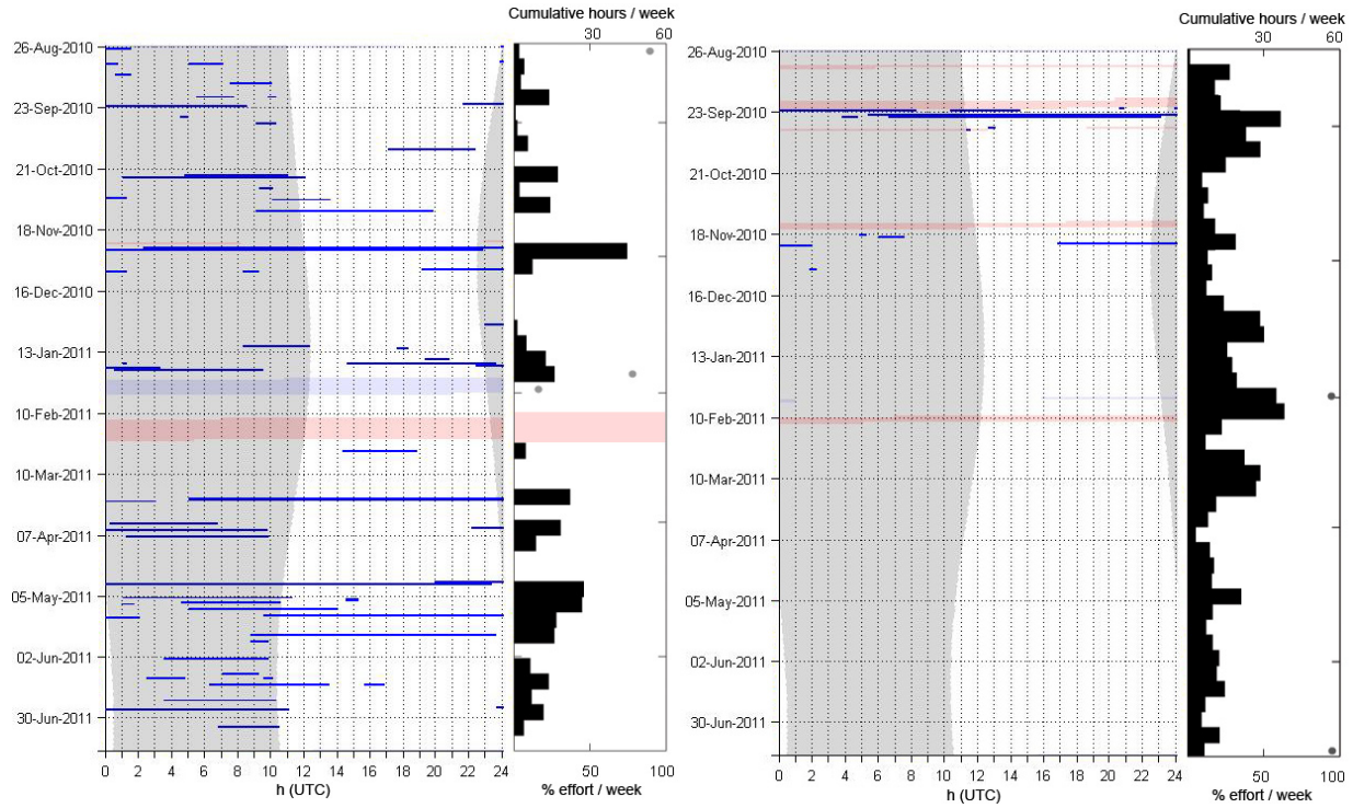
Figure 47. CT27 echolocation clicks in one-minute bins (blue) and weekly presence (black) at site A (left) and site B (right) between August 2010 and July 2011. Red shading indicates data gaps. Gray shading is nighttime.
