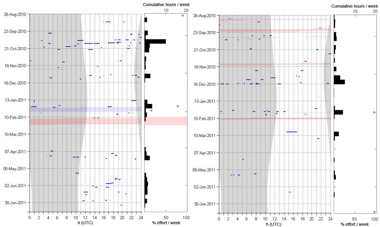
Figure 54. Echosounder pings in one-minute bins (blue) and weekly echosounder presence (black) at site A (left) and site B (right) between August 2010 and July 2011.
