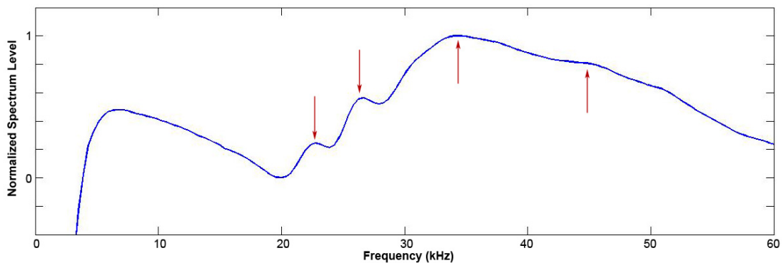
Figure 18. Risso's dolphin echolocation click mean spectra. Arrows show locate spectral peaks.
