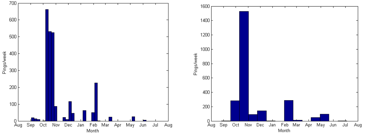
Figure 51. Mid-Frequency Active (MFA) sonar presence in weekly bins at site A (left panel) and site B (right panel) between August 2010 and July 2011.
