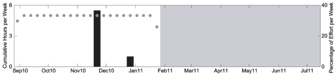
Figure 40. Weekly occurrence of downsweep calls in site A. Effort as described in Figure 37
