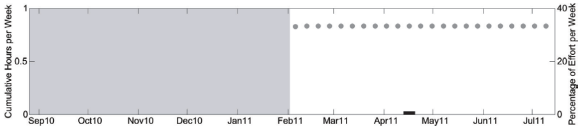
Figure 42. Weekly presence of all humpback whale calls (black bars) at site B between February and July 2011. No humpback calls were recorded at site A. Effort as described in Figure 37
