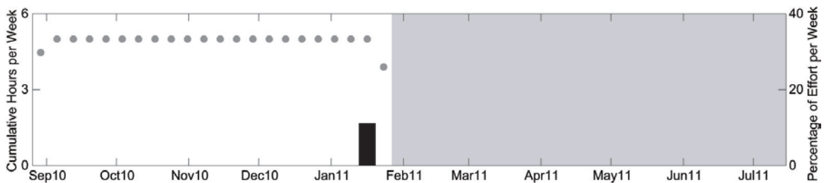
Figure 38. Occurrence of minke whale 50 Hz pulses at site A. Effort as described in Figure 37
