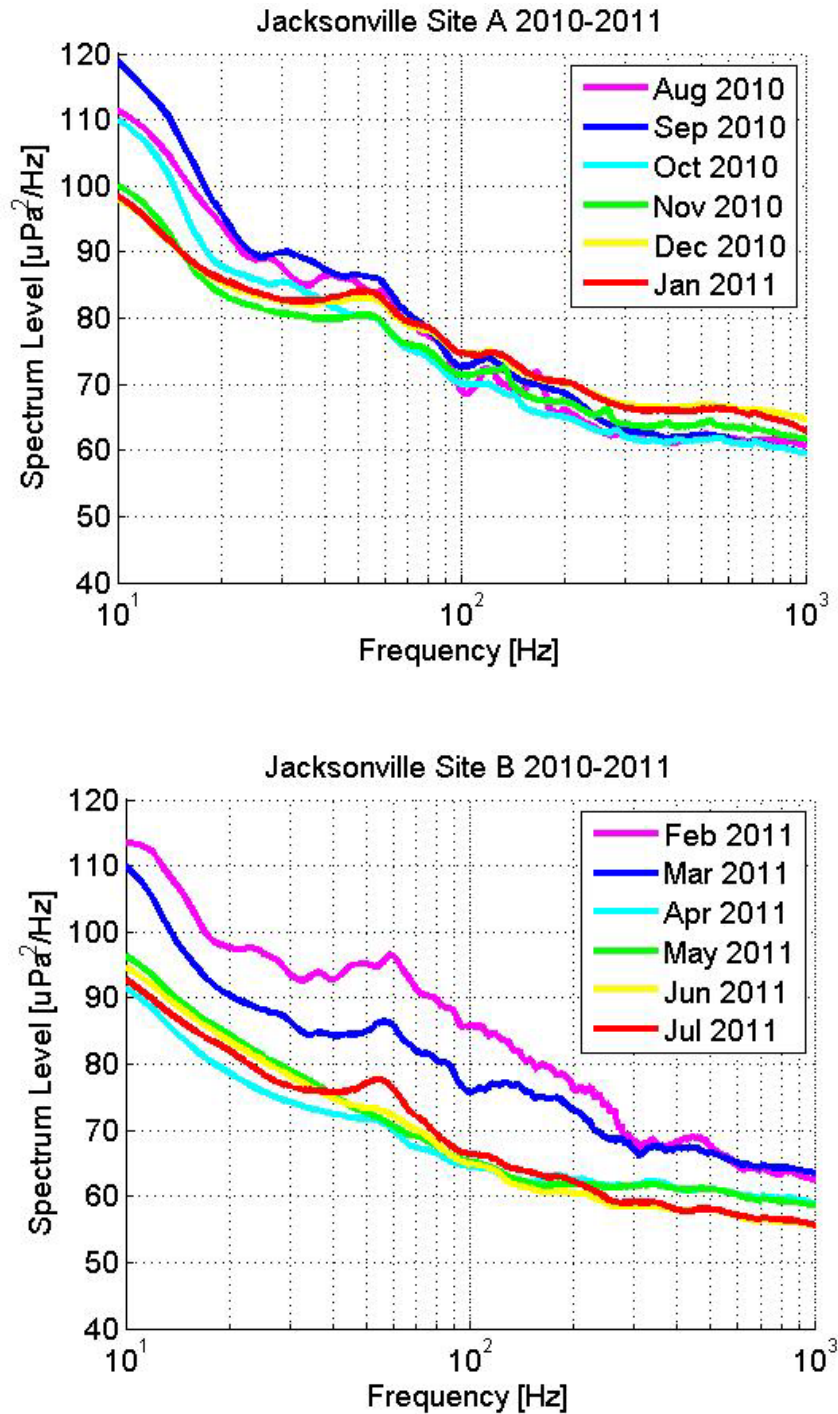
Figure 36. Monthly averages of ambient noise at site A (above) and site B (below) for the period August 2010 – July 2011. Legend gives color-coding by date.
