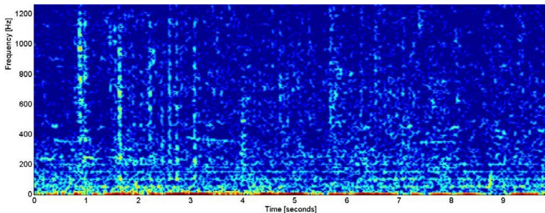
Figure 13. Humpback whale calls recorded at site A on April 13, 2011.
