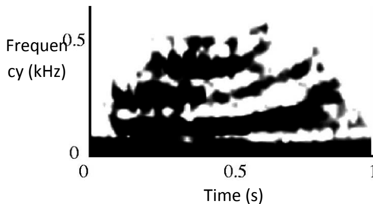
Figure 11. Right whale upcall call from Parks and Tyack (2005).
