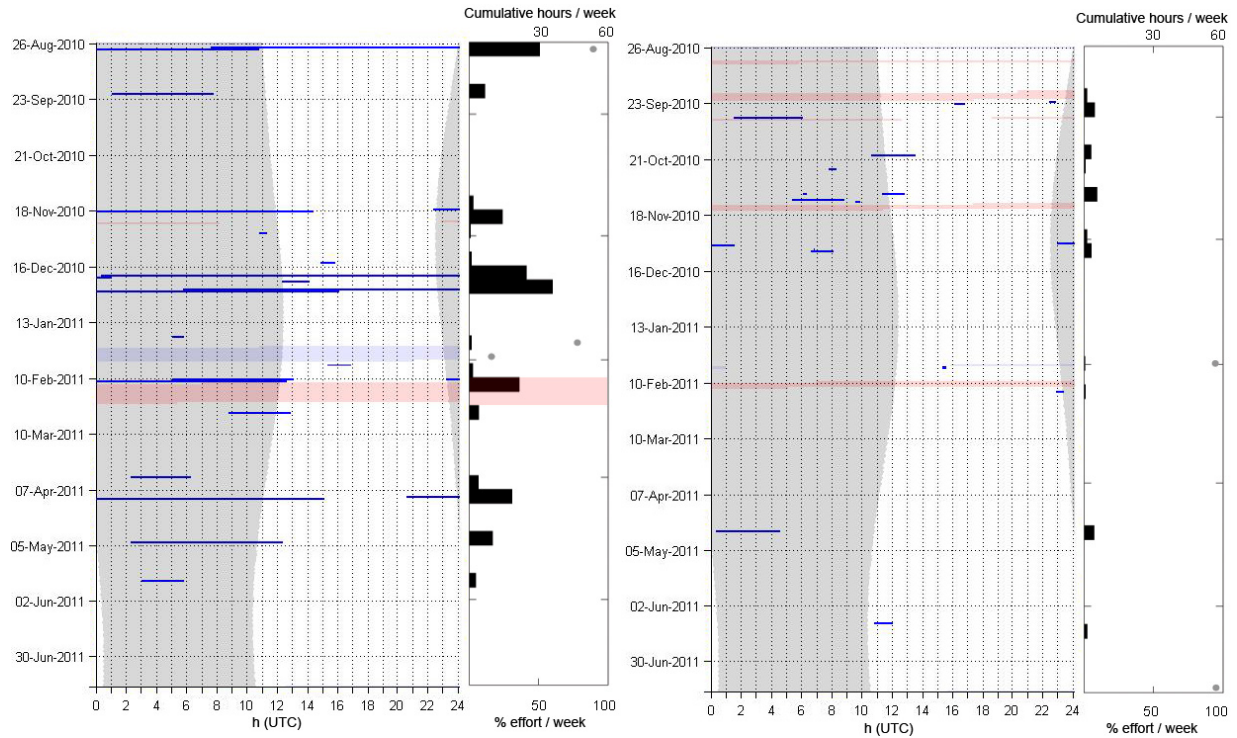
Figure 45. CT25 echolocation clicks in one-minute bins (blue) and weekly presence (black) at site A (left) and site B (right) between August 2010 and July 2011. Red shading indicates data gaps. Gray shading is nighttime.
