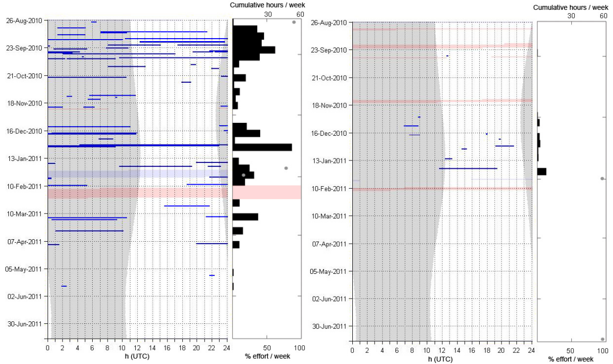
Figure 49. CT32 echolocation clicks in one-minute bins and weekly presence at site A (left) and site B (right) between August 2010 and July 2011. Red shading indicates data gaps. Gray shading is nighttime.
