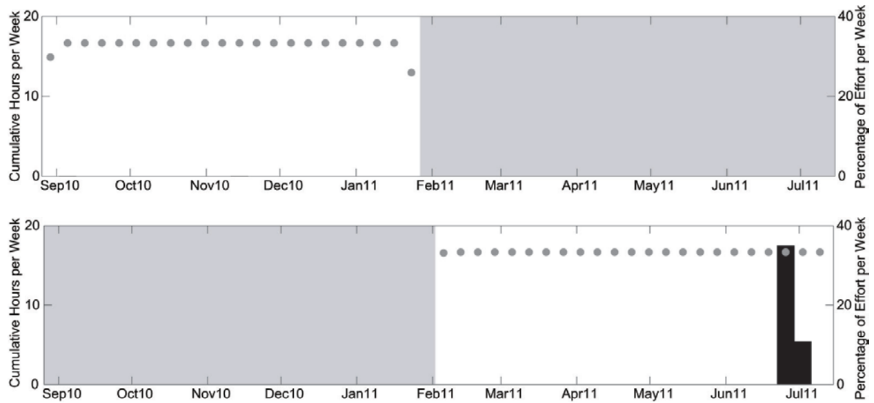
Figure 55. Weekly hours with explosions at sites A (top) and B (bottom) between August 2010 and July 2011. Effort markings are as described in Figure 37.
