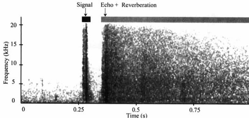
Figure 14. North Atlantic Right whale gunshot call from Parks et al. , 2005.
