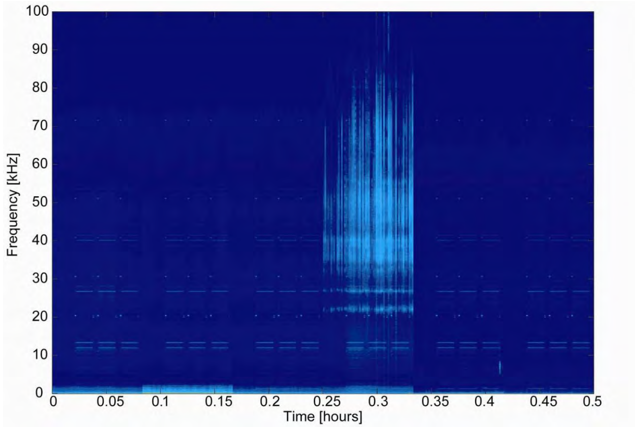
Figure 9. Pacific white-sided dolphin echolocation clicks in a LTSA.
