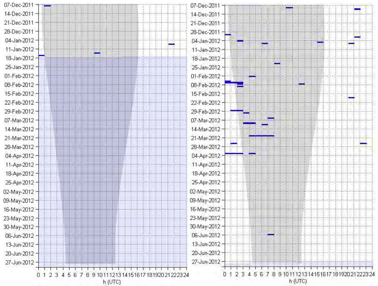
Blue whale –D call in hourly bins at sites CE (left) and QC (right).
