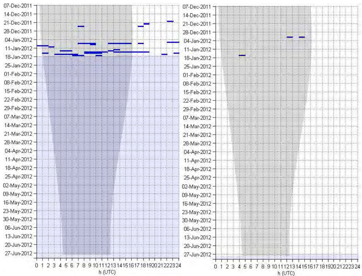
Gray whale – Calls in hourly bins at sites CE (left) and QC (right).
