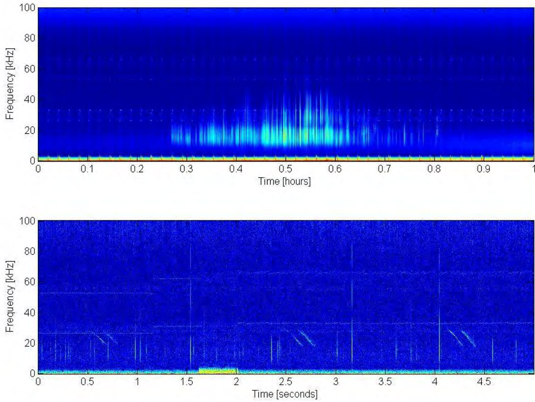
Figure 10. Killer whale echolocation clicks and HFM signals in a LTS (top) and spectrogram (bottom).
