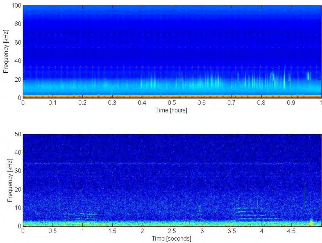
Figure 11. Killer whale pulsed calls in a LTS (top) and spectrogram (bottom).
