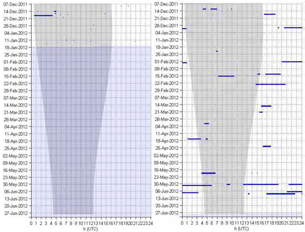
Sperm whale – Echolocation clicks in five-minute bins at sites CE (left) and QC (right).
