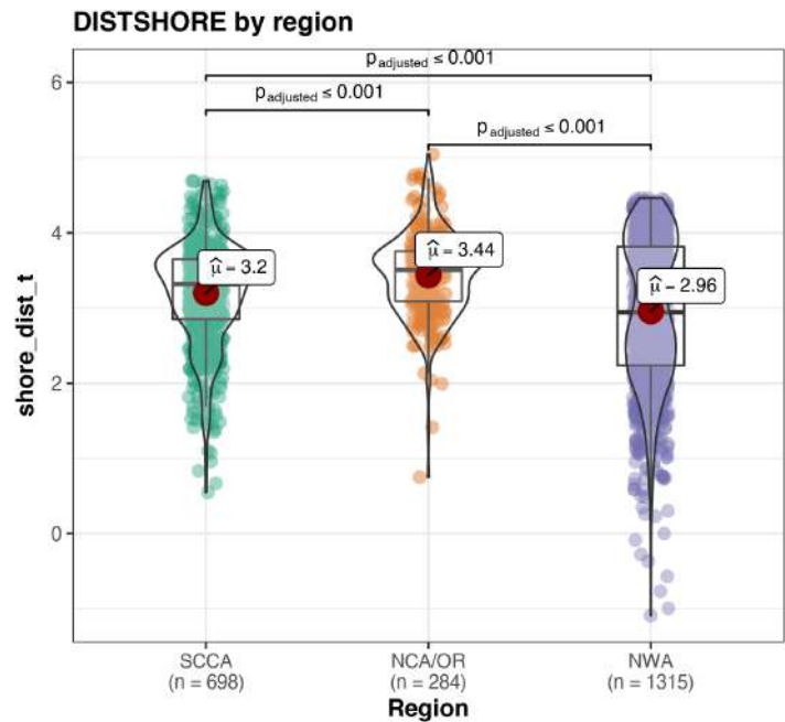
Figure 59. Box-violin plots showing the distributional characteristics of DISTSHELF (km) and DISTSORE (km) for SSSM/hSSSM locations (ARS mode only) in each tagging region (SCCA = southern and central California, NCA/OR = northern California/Oregon, NWA = northern Washington). Red circles indicate the mean. The y-axis has been log-transformed to enhance visualization and for formal statistical testing. Pairwise comparisons based on Yuen's test on trimmed means and adjusted for multiple p-values are shown, as implemented in R package ggstatsplot v. 0.5.0.9000 (Patil 2018).
