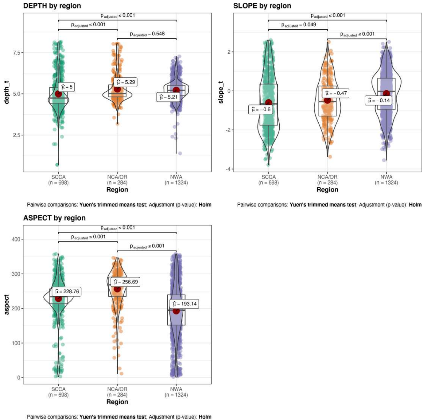
Figure 58. Box-violin plots showing the distributional characteristics of DEPTH (m), SLOPE (deg), and ASPECT (deg) for SSSM/hSSSM locations (ARS mode only) in each tagging region (SCCA = southern and central California, NCA/OR = northern California/ Oregon, NWA = northern Washington). Red circles indicate the mean. The y-axis has been log-transformed for DEPTH and SLOPE to enhance visualization and for formal statistical testing. Pairwise comparisons based on Yuen's test on trimmed means and adjusted for multiple p -values are shown, as implemented in R package ggstatsplot v. 0.5.0.9000 (Patil 2018).
