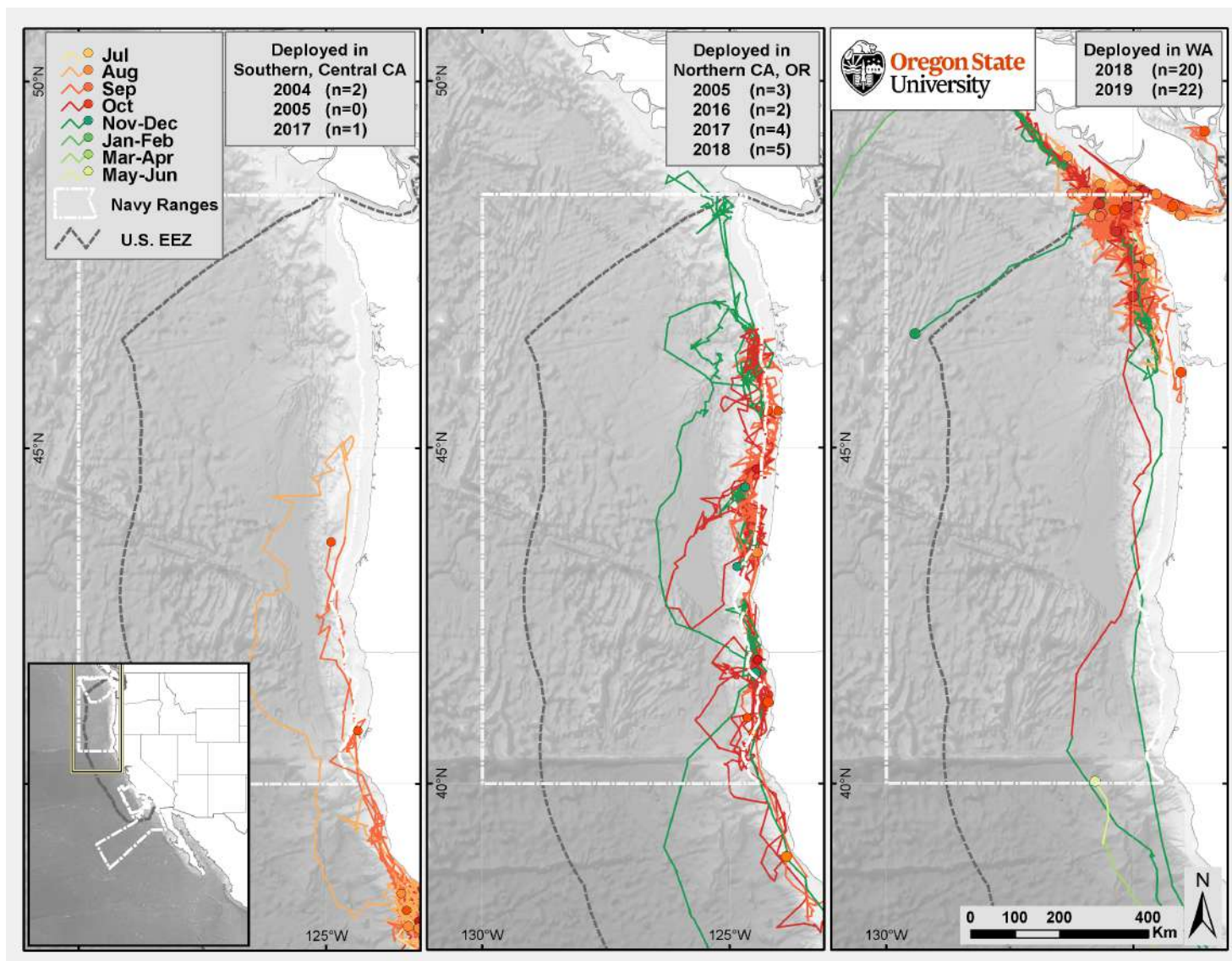
Figure 26. Satellite-monitored tracks in NWTT for humpback whales tagged in SCCA in 2004, 2005, and 2017 (3 tags; left panel), in NCA/OR in 2005 and 2016 to 2018 (14 tags; middle panel), and in NWA in 2018 and 2019 (42 tags; right panel).
