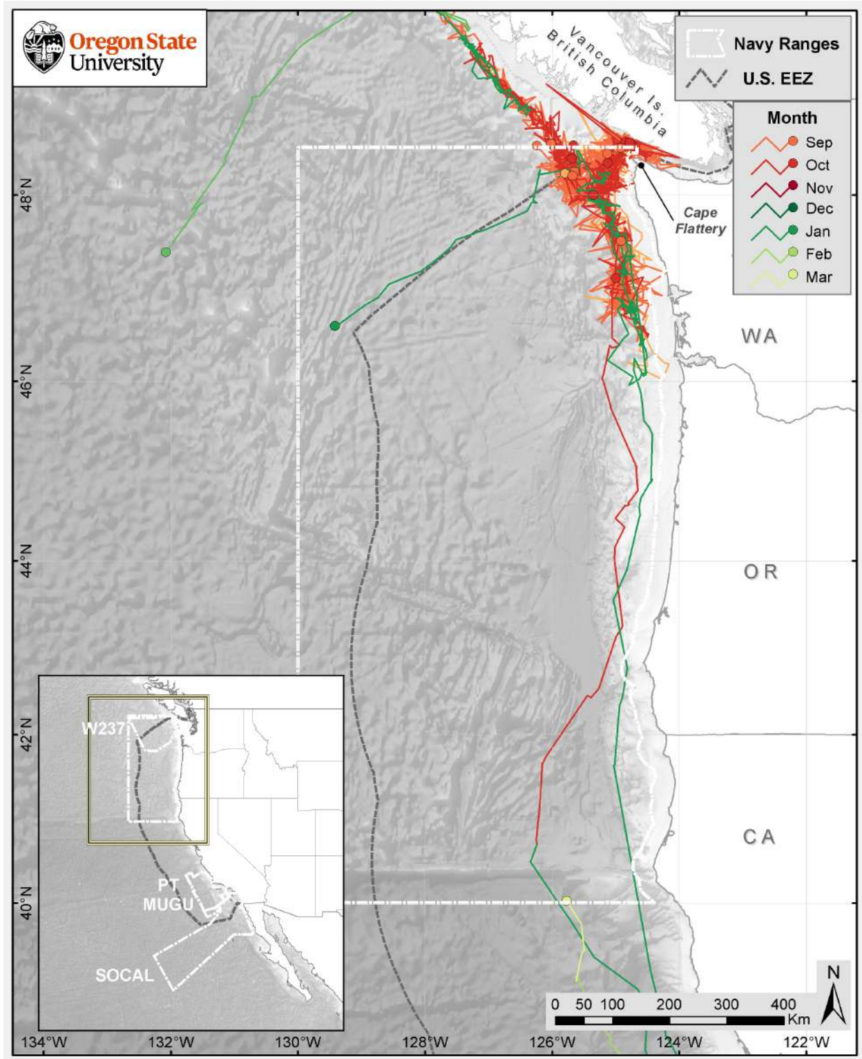
Figure 10. Satellite-monitored tracks in NWT for humpback whales tagged off Washington in September and October 2019 (22 DM tags).
