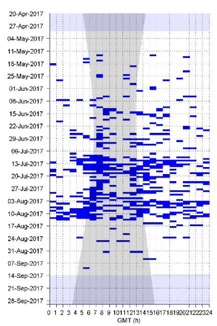
Figure 23. Diel presence of blue whale D calls, indicated by blue dots, in one hour bins at sites CB (left), AB (middle), and QN (right). Gray vertical shading denotes nighttime and gray horizontal shading denotes absence of acoustic data.
