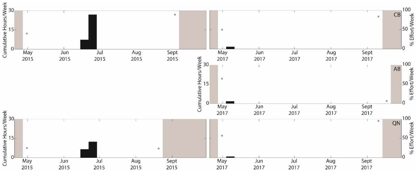
Figure 38. Weekly presence of MFA sonar <5kHz from May to September 2015 and April to September 2017 at sites CB (top), AB (middle), and QN (bottom). Gray dots represent the percent of effort per week in weeks with less than 100% recording effort, and gray shading represents periods with no recording effort. Where gray dots or shading are absent, full recording effort occurred for the entire week.
