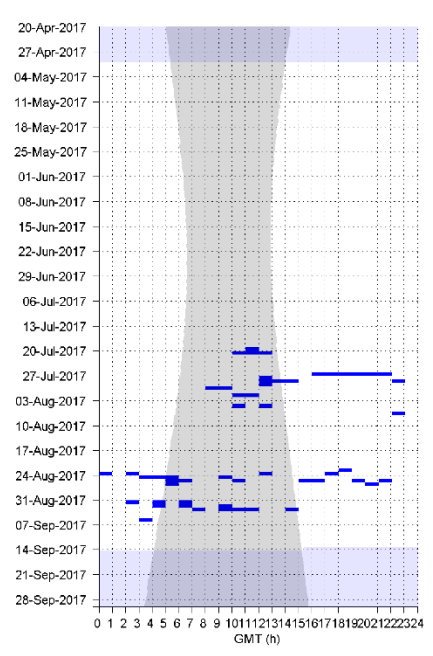
Figure 21. Diel presence of Central Pacific tonal blue whale calls, indicated by blue dots, in one hour bins at sites CB (left), AB (middle), and QN (right). Gray vertical shading denotes nighttime and gray horizontal shading denotes absence of acoustic data.
