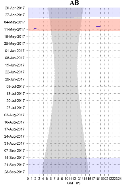
Figure 39. Naval training events (shaded red) overlaid on diel presence of MFA sonar <5kHz signals, indicated by blue dots, in one minute bins at sites CB (left), AB (middle), and QN (right). Gray vertical shading denotes nighttime and gray horizontal shading denotes absence of acoustic data.
