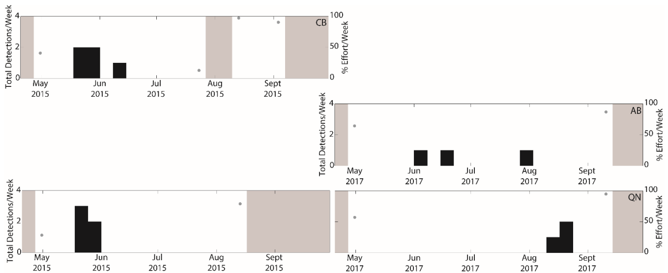
Figure 47. Weekly presence of explosions from May to September 2015 and April to September 2017 at sites CB (top), AB (middle), and QN (bottom). There were no explosion detections in 2017 at site CB. Gray dots represent the percent of effort per week in weeks with less than 100% recording effort, and gray shading represents periods with no recording effort. Where gray dots or shading are absent, full recording effort occurred for the entire week.
