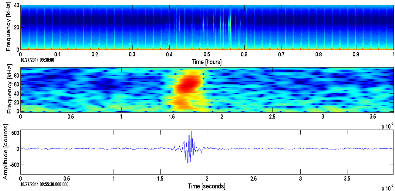
Figure 13. Echolocation sequence of Stejneger's beaked whale in an LTSA (top) and single FM pulse in a spectrogram (middle) and timeseries (bottom) previously recorded at site QN.
