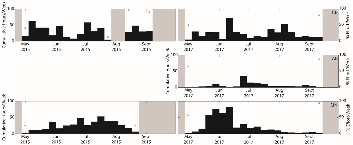
Figure 25. Weekly presence of fin whale 40 Hz calls from May to September 2015 and April to September 2017 at sites CB (top), AB (middle), and QN (bottom). Gray dots represent the percent of effort per week in weeks with less than 100% recording effort, and gray shading represents periods with no recording effort. Where gray dots or shading are absent, full recording effort occurred for the entire week.
