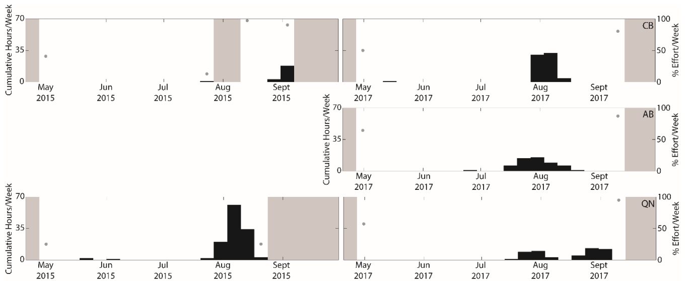
Figure 20. Weekly presence of Central Pacific tonal blue whale calls from May to September 2015 and April to September 2017 at sites CB (top), AB (middle), and QN (bottom). Gray dots represent the percent of effort per week in weeks with less than 100% recording effort, and gray shading represents periods with no recording effort. Where gray dots or shading are absent, full recording effort occurred for the entire week.
