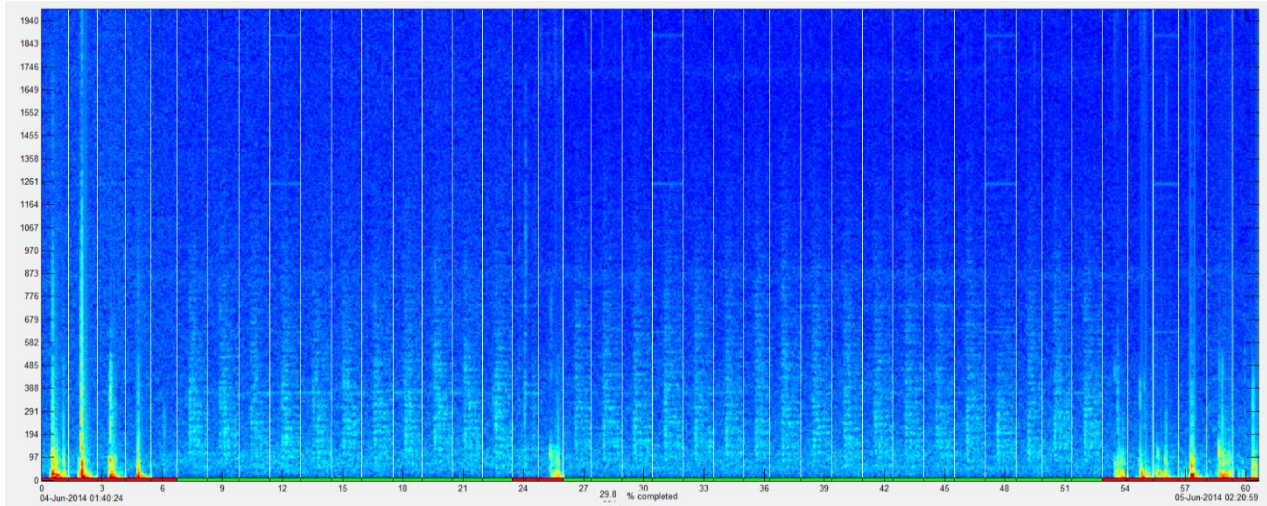
Figure 16. Explosions in the analyst verification stage of the detector previously recorded at site PT. Green in the bottom evaluation line indicates true and red indicates false detections.
