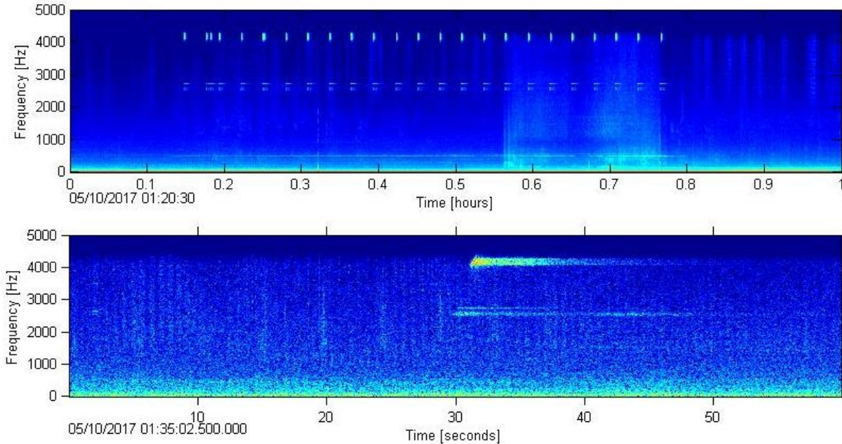
Figure 14. Mid-frequency Active (MFA) sonar in an LTSA (top) and spectrogram (bottom) recorded at site CB.
