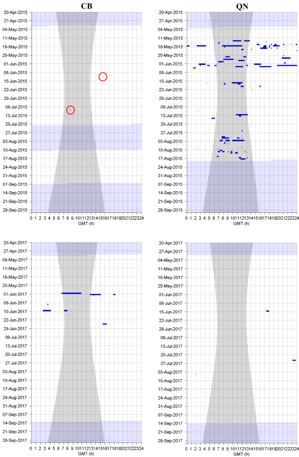
Figure 30. Diel presence of humpback whale calls, indicated by blue dots, in one minute bins at sites CB (left) and QN (right). There were no detections of humpback whale calls at site AB in 2017. Gray vertical shading denotes nighttime and gray horizontal shading denotes absence of acoustic data.
