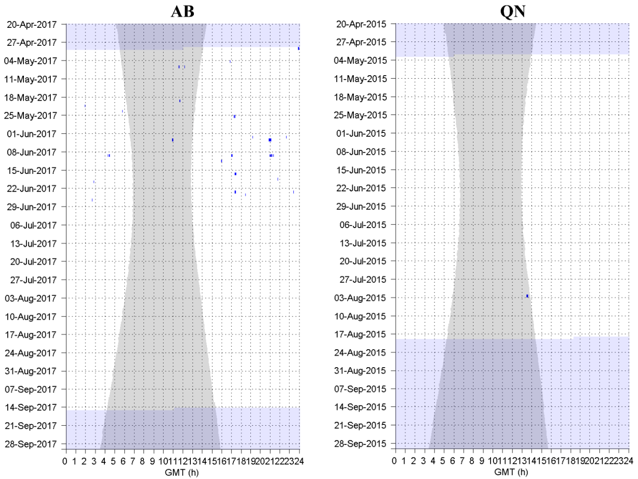
Figure 35. Diel presence of Cuvier’s beaked whale FM pulses, indicated by blue dots, in one minute bins at site AB (left) and in five minute bins at site QN (right). There were no detections of Cuvier’s at site CB or in 2017 at site QN. Gray vertical shading denotes nighttime and gray horizontal shading denotes absence of acoustic data.
