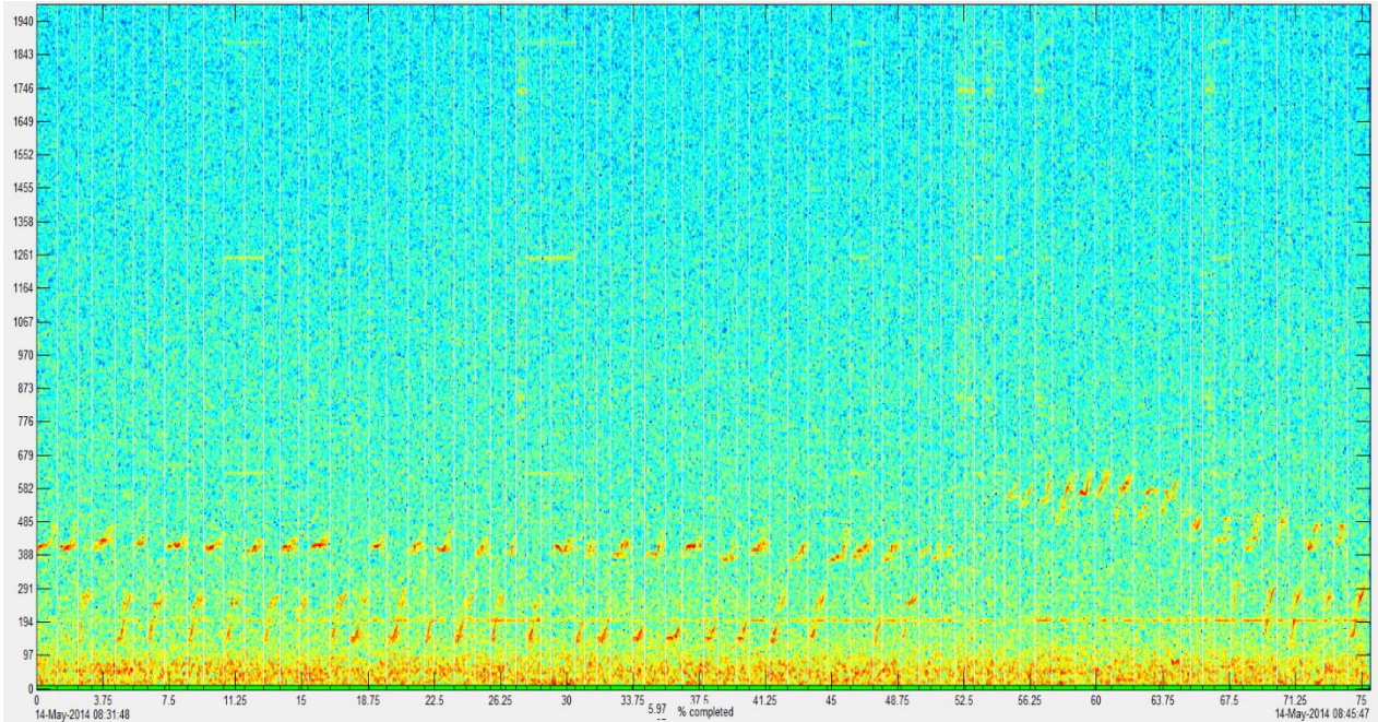
Figure 9. Humpback whale song shown in the analyst verification stage of the detector previously recorded at site KO.
