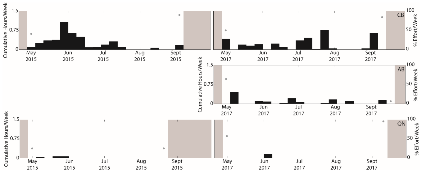
Figure 36. Weekly presence of Stejneger's beaked whale FM pulses between May 2015 and September 2017 at sites CB (top), AB (middle), and QN (bottom).
