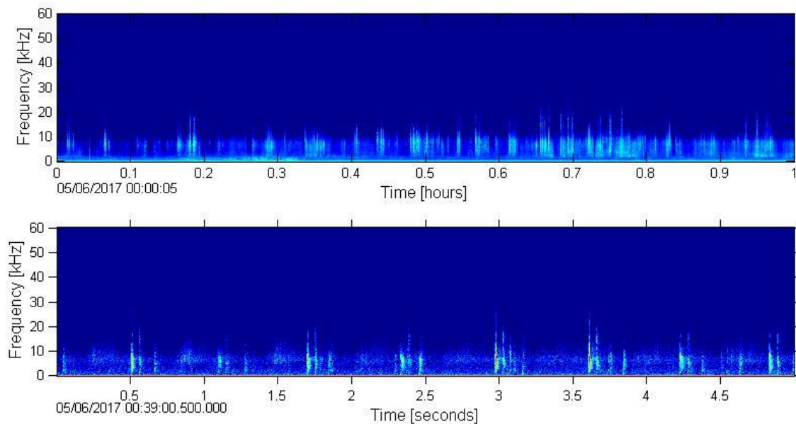
Figure 11. Sperm whale echolocation clicks in an LTSA (top) and spectrogram (bottom) recorded at site CB.
