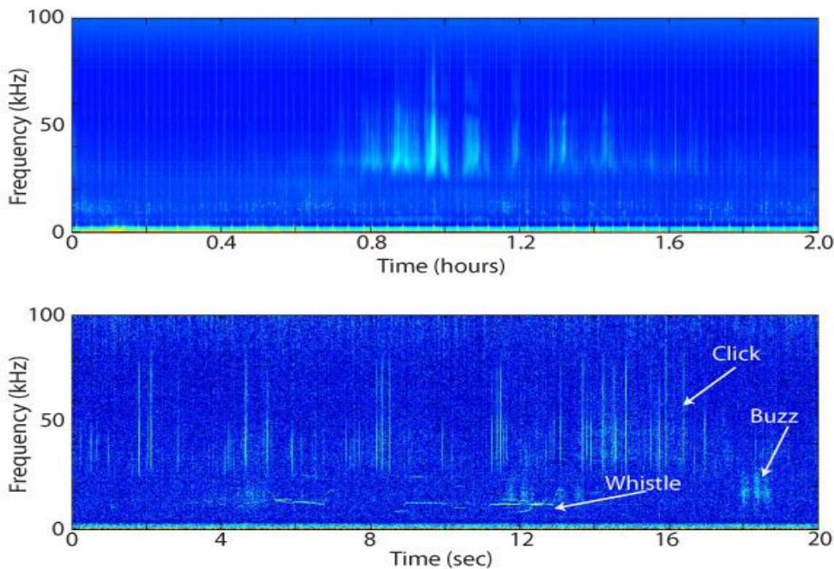
Figure 10. LTSA (top) and spectrogram (bottom) demonstrating odontocete signal types.
