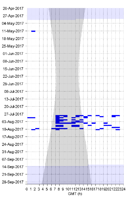
Figure 21. Diel presence of Central Pacific tonal blue whale calls, indicated by blue dots, in one hour bins at sites CB (left), AB (middle), and QN (right). Gray vertical shading denotes nighttime and gray horizontal shading denotes absence of acoustic data.
