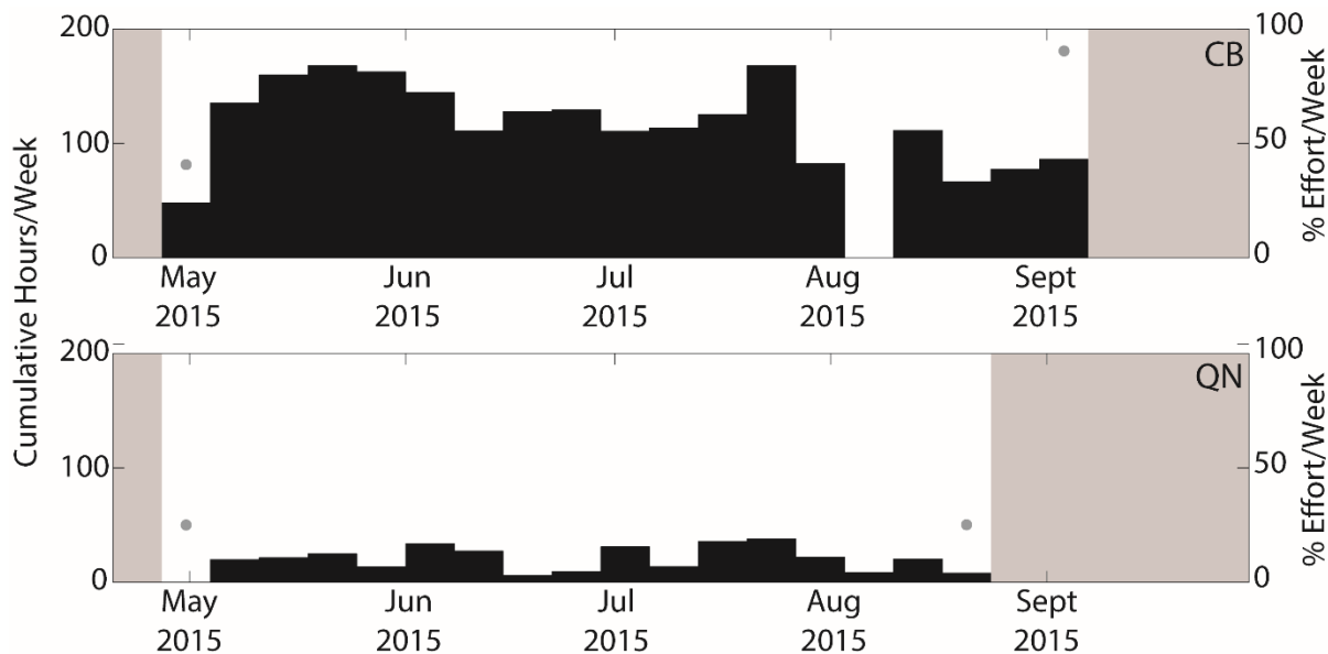
Figure 31. Weekly presence of sperm whale clicks between May and September 2015 at sites CB (top) and QN (bottom).
