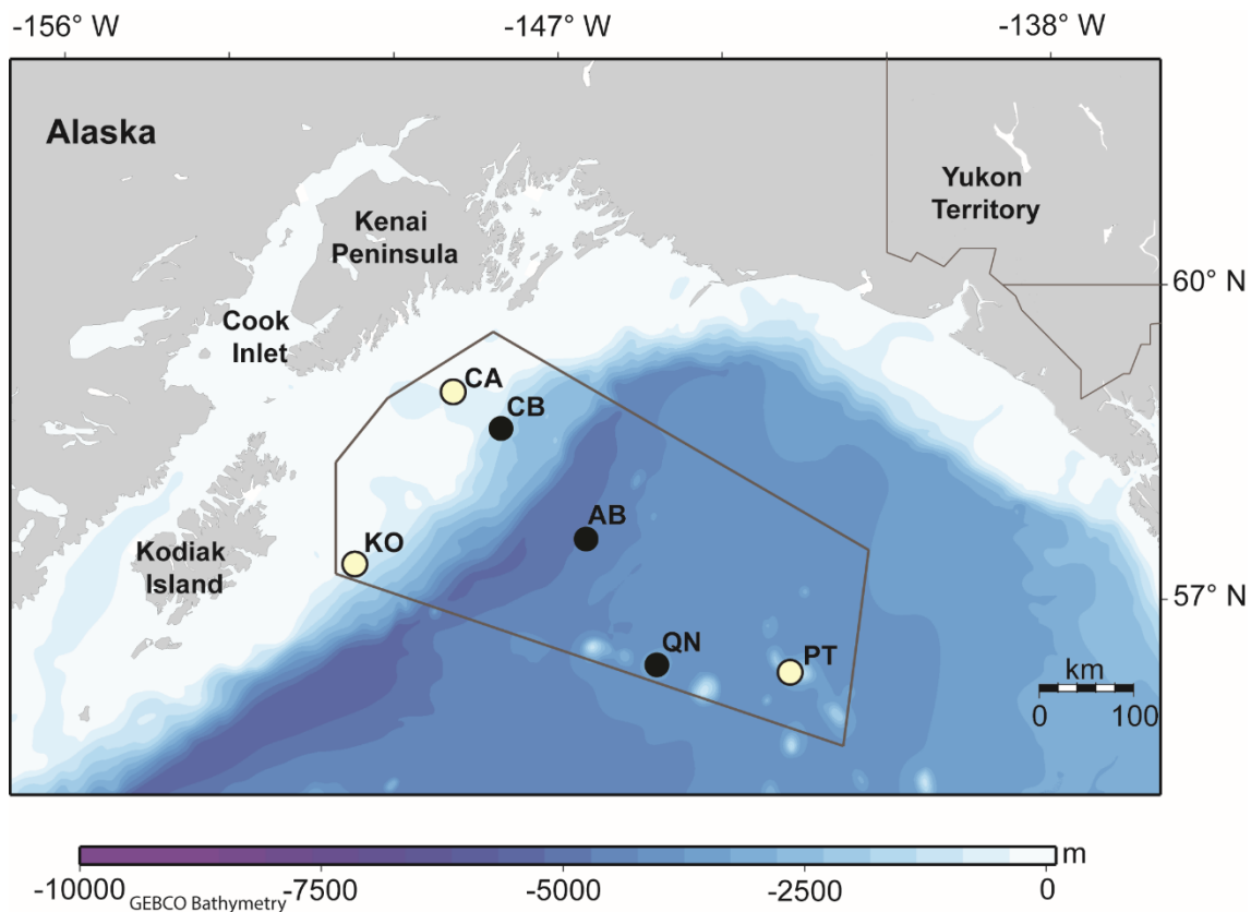
Figure 1. Locations of current (black circles) and previous (white circles) High-frequency Acoustic Recording Package (HARP) deployment sites in the GATMAA (gray line). Only sites CB and QN were monitored from May to September 2015; whereas CB, AB, and QN were monitored from April to September 2017.
