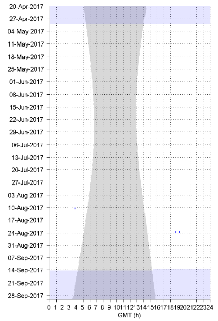
Figure 48. Diel presence of explosion detections, indicated by blue dots, in five-minute bins at sites CB (left), AB (middle), and QN (right). There were no explosion detections in 2017 at site CB. Gray vertical shading denotes nighttime and gray horizontal shading denotes absence of acoustic data.
