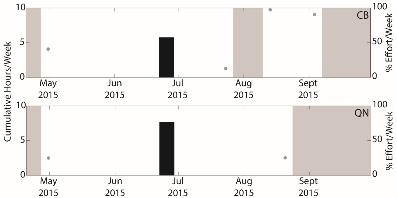
Figure 45. Weekly presence of LFA sonar >500Hz between May and September 2015 at sites CB (top) and QN (bottom). There was no LFA presence at any site in 2017. Gray dots represent the percent of effort per week in weeks with less than 100% recording effort, and gray shading represents periods with no recording effort. Where gray dots or shading are absent, full recording effort occurred for the entire week.
