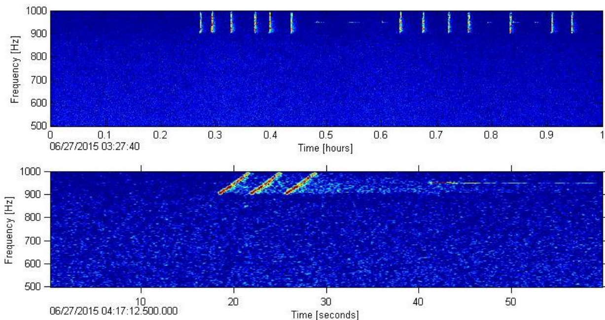
Figure 15. Low-frequency Active (LFA) sonar in an LTSA (top) and a spectrogram (bottom) recorded at site CB.
