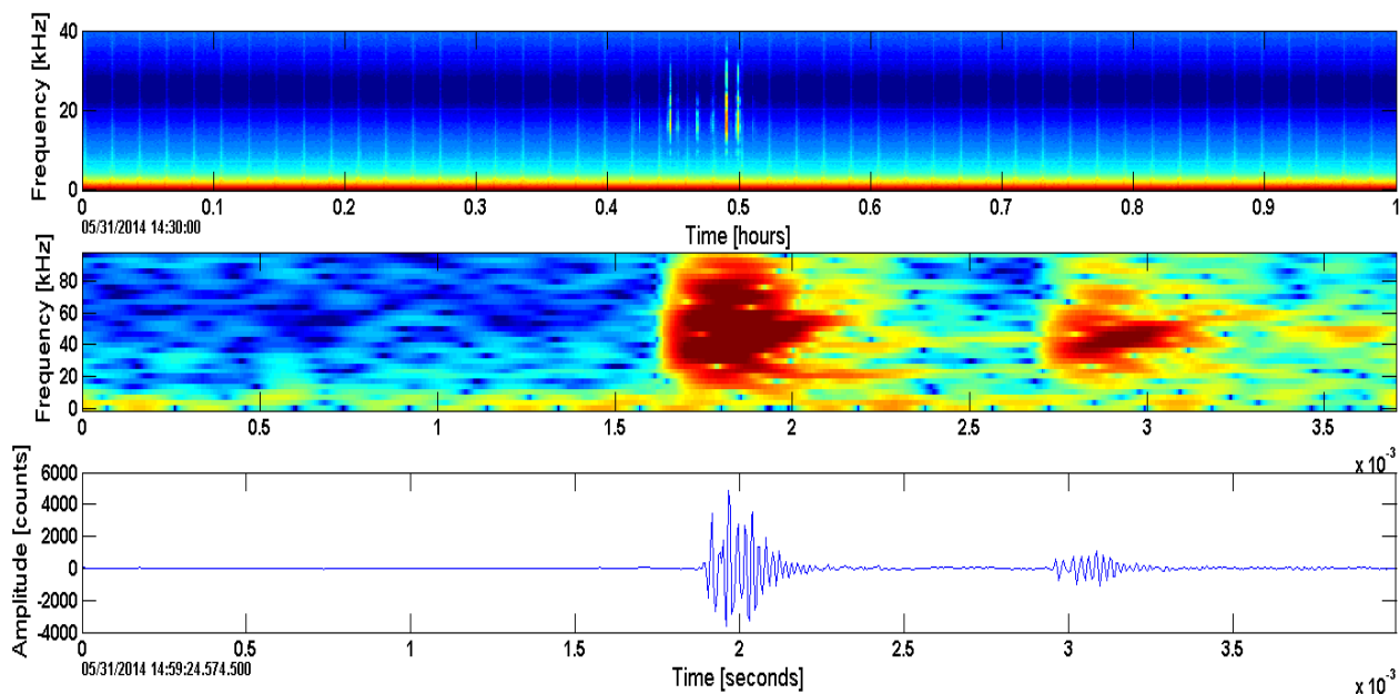
Figure 12. Echolocation sequence of Cuvier's beaked whale in an LTSA (top) and an example FM pulse in a spectrogram (middle) and timeseries (bottom) previously recorded at site PT.
