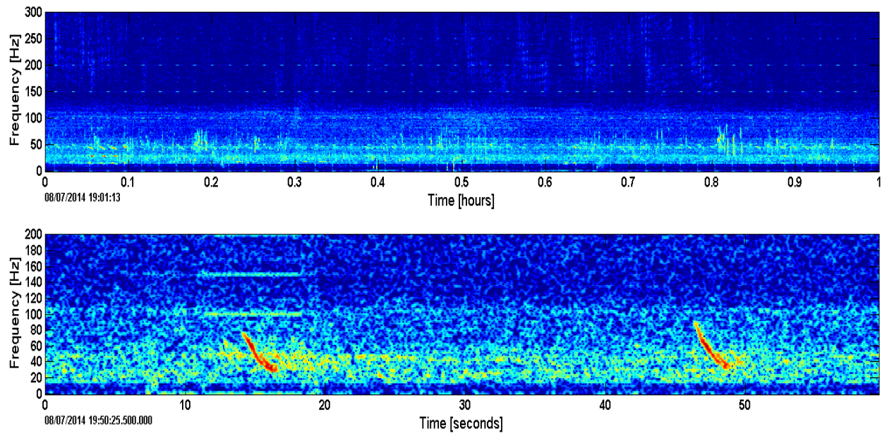
Figure 4. Blue whale D calls (around 50 Hz) in an LTSA (top) and two individual calls shown in a spectrogram (bottom) previously recorded at site CB.
