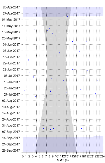
Figure 37. Diel presence of Stejneger's beaked whale FM pulses, indicated by blue dots, in one minute bins at sites CB (left), AB (middle), and QN (right). Gray vertical shading denotes nighttime and gray horizontal shading denotes absence of acoustic data.
