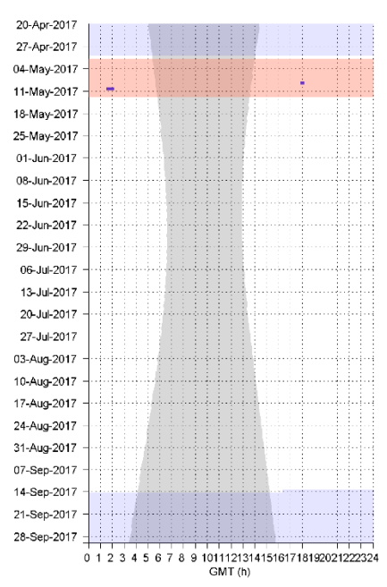
Figure 39. Naval training events (shaded red) overlaid on diel presence of MFA sonar <5kHz signals, indicated by blue dots, in one minute bins at sites CB (left), AB (middle), and QN (right). Gray vertical shading denotes nighttime and gray horizontal shading denotes absence of acoustic data.
