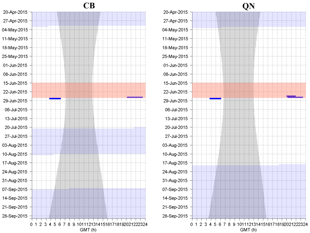
Figure 46. Major naval training events (shaded red) overlaid on diel presence of LFA sonar >500Hz signals, indicated by blue dots, in one minute bins at sites CB (left) and QN (right). There was no LFA presence in 2017. Gray vertical shading denotes nighttime and gray horizontal shading denotes absence of acoustic data.
