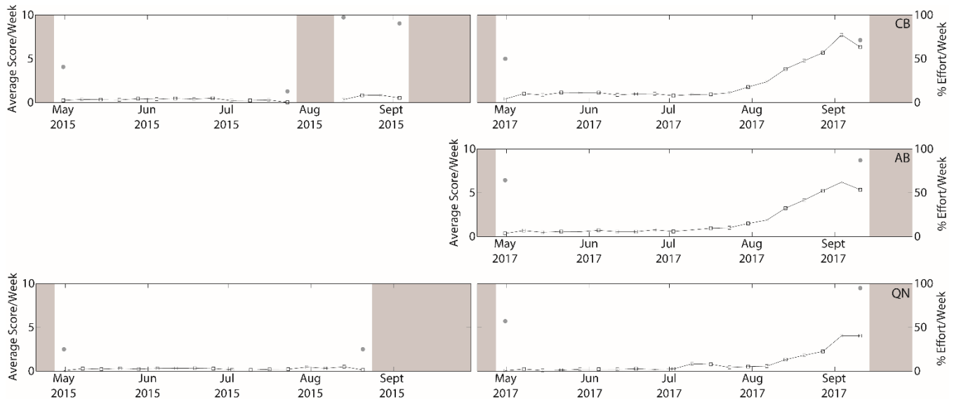
Figure 24. Weekly presence of fin whale acoustic index (proxy for 20 Hz calls) from May to September 2015 and April to September 2017 at sites CB (top), AB (middle), and QN (bottom).
