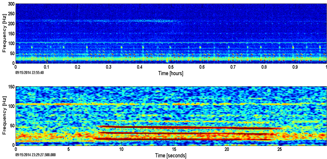
Figure 2. Northeast Pacific blue whale B calls (just below 50 Hz) in Long-term Spectral Average (LTSA; top) and an individual call shown in a spectrogram (bottom) previously recorded at site CB.
