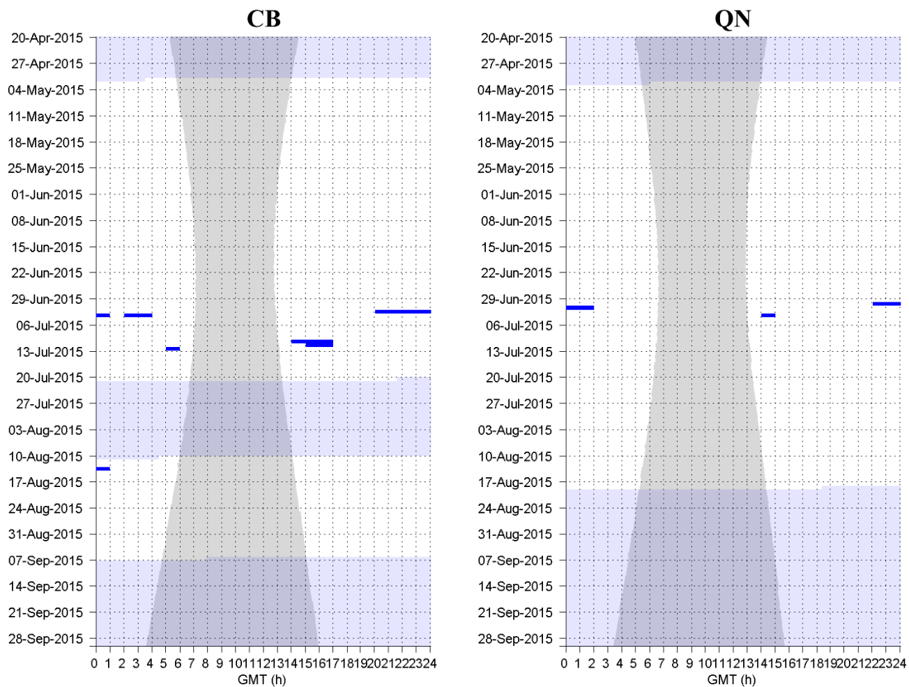
Figure 28. Diel presence of gray whale M3 calls, indicated by blue dots, in one hour bins at sites CB (left) and QN (right) in 2015. There were no M3 detections at any site in 2017. Gray vertical shading denotes nighttime and gray horizontal shading denotes absence of acoustic data.
