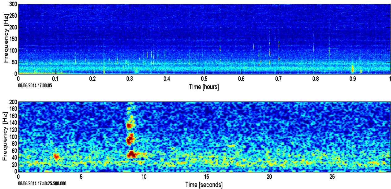
Figure 7. Gray Whale M3 calls in an LTSA (top) and an individual call shown in a spectrogram (bottom) previously recorded at site KO.
