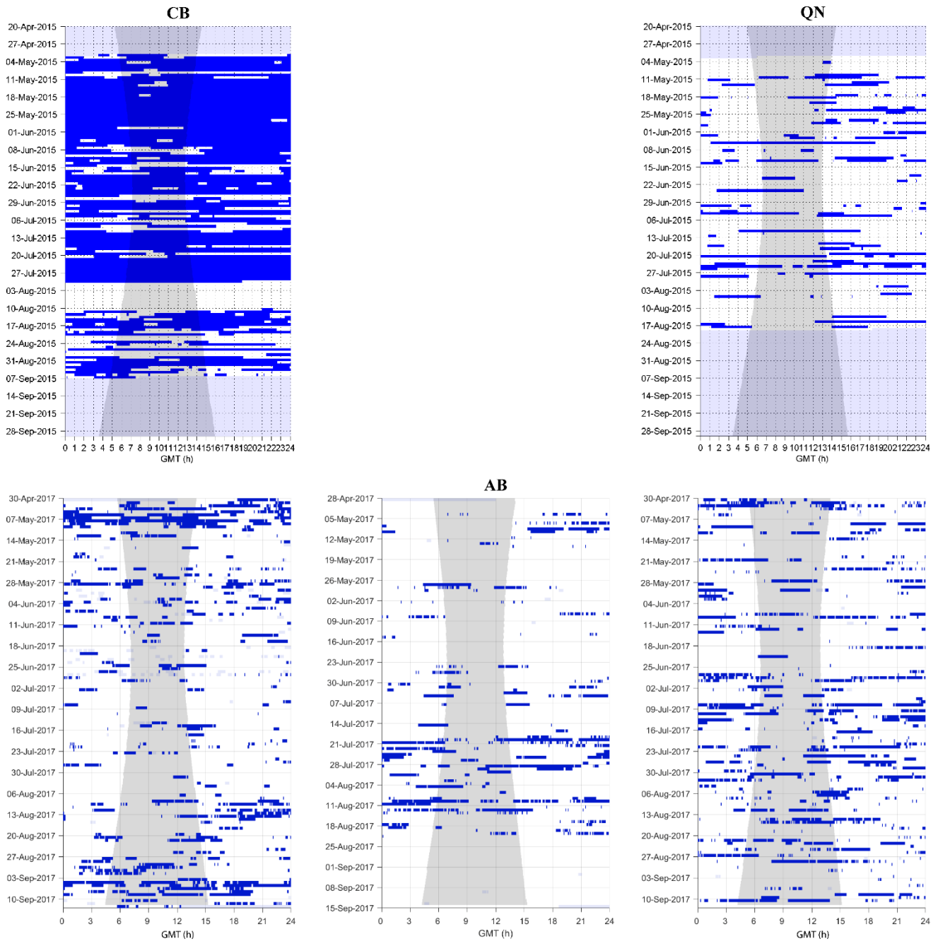
Figure 33. Diel presence of sperm whale clicks, indicated by blue dots, in one minute bins at site CB (left), AB (middle), and QN (right). Detections in 2015 were logged as encounters in 2015 and individual clicks in 2017. Gray vertical shading denotes nighttime and gray horizontal shading denotes absence of acoustic data.
