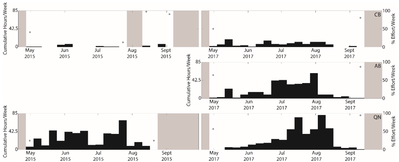
Figure 22. Weekly presence of blue whale D calls from May to September 2015 and April to September 2017 at sites CB (top), AB (middle), and QN (bottom). Gray dots represent the percent of effort per week in weeks with less than 100% recording effort, and gray shading represents periods with no recording effort. Where gray dots or shading are absent, full recording effort occurred for the entire week.
