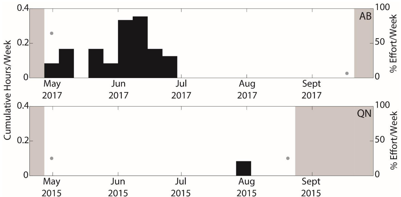
Figure 34. Weekly presence of Cuvier's beaked whale FM pulses from May to September 2015 and April to September 2017 at sites AB (top) and QN (bottom). There were no detections of Cuvier's at site CB or in 2017 at site QN.
