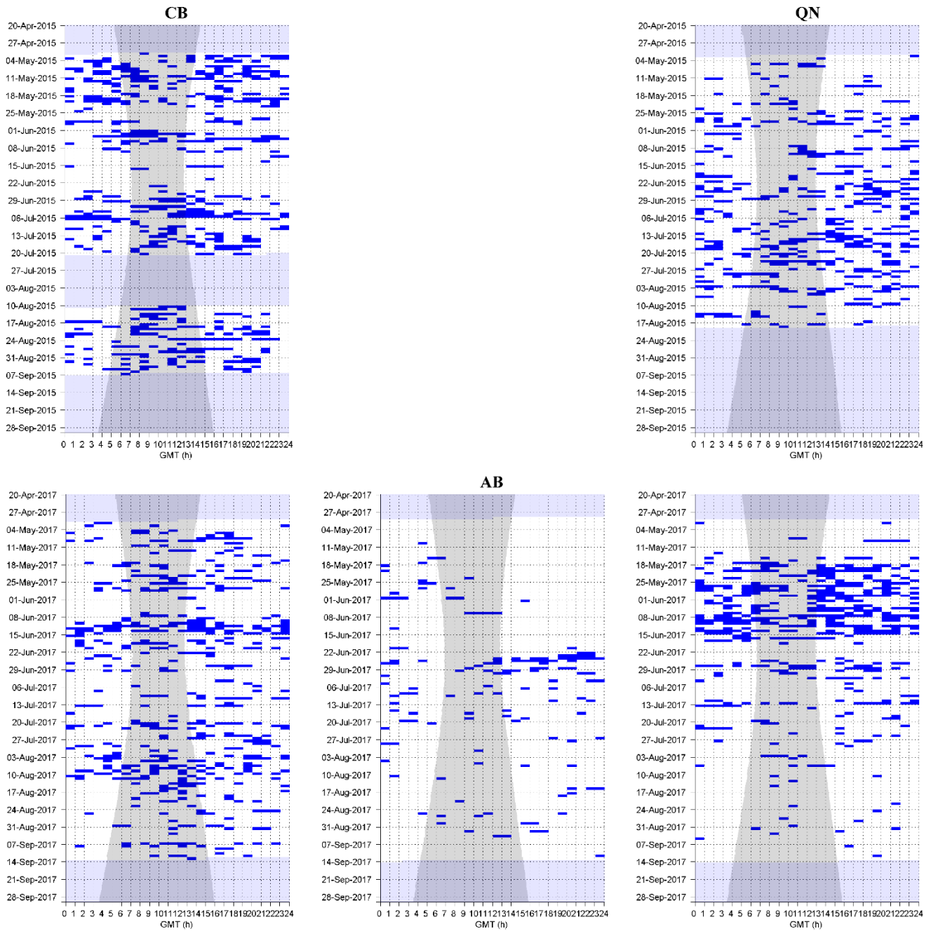
Figure 26. Diel presence of fin whale 40 Hz calls, indicated by blue dots, in one hour bins at sites CB (left), AB (middle), and QN (right). Gray vertical shading denotes nighttime and gray horizontal shading denotes absence of acoustic data.
