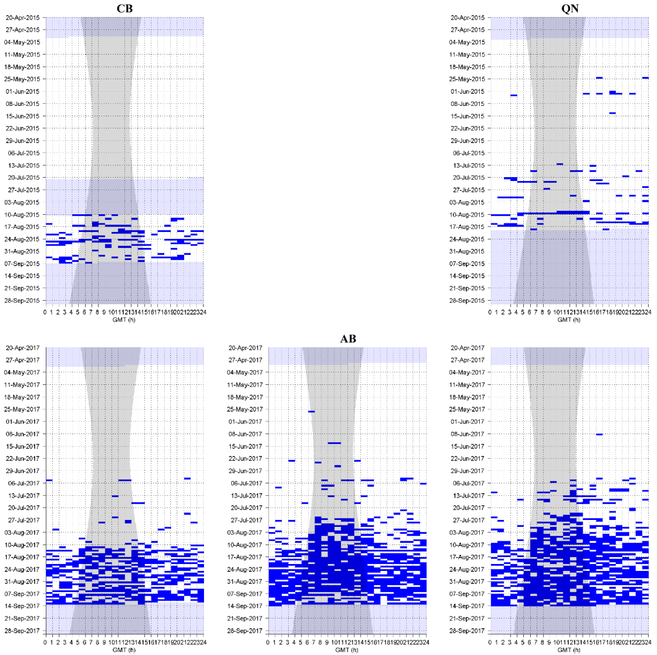
Figure 19. Diel presence of NE Pacific blue whale B calls, indicated by blue dots, in one hour bins at sites CB (left), AB (middle), and QN (right). Gray vertical shading denotes nighttime and gray horizontal shading denotes absence of acoustic data.
