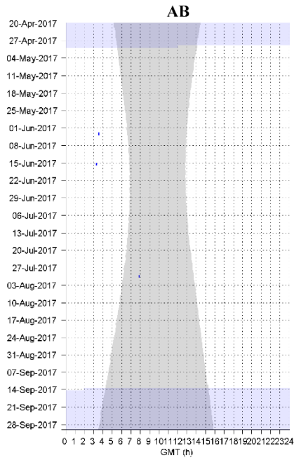
Figure 48. Diel presence of explosion detections, indicated by blue dots, in five-minute bins at sites CB (left), AB (middle), and QN (right). There were no explosion detections in 2017 at site CB. Gray vertical shading denotes nighttime and gray horizontal shading denotes absence of acoustic data.
