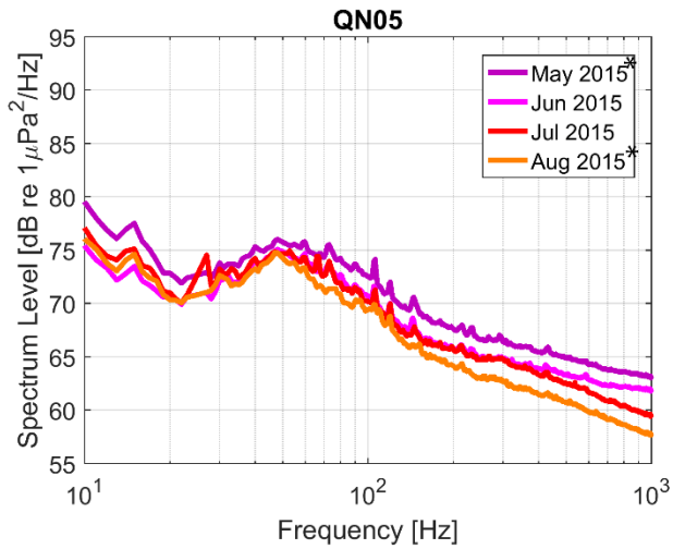
Figure 17. Monthly average sound spectrum levels at sites CB (top), AB (middle), and QN (bottom). Legend gives color-coding by month. * denotes months with partial effort.
