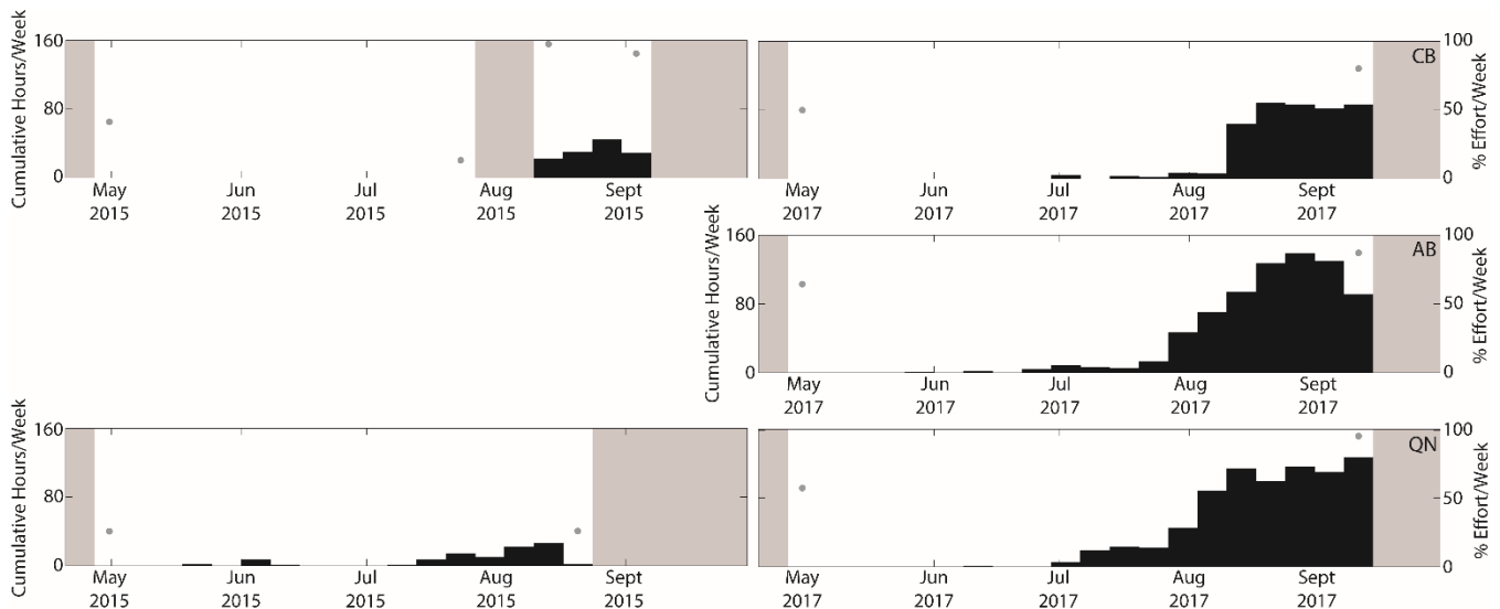
Figure 18. Weekly presence of NE Pacific blue whale B calls from May to September 2015 and April to September 2017 at sites CB (top), AB (middle), and QN (bottom).
